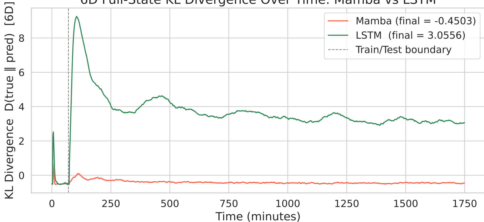
6D Full-State KL Divergence Over Time: Mamba vs LSTM
