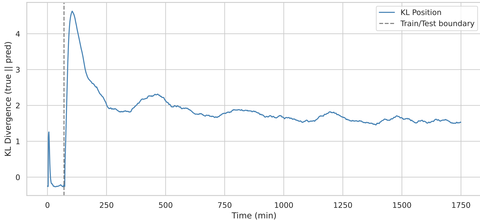
Final Position KL Divergence: lstm — Pos KL=1.5280
