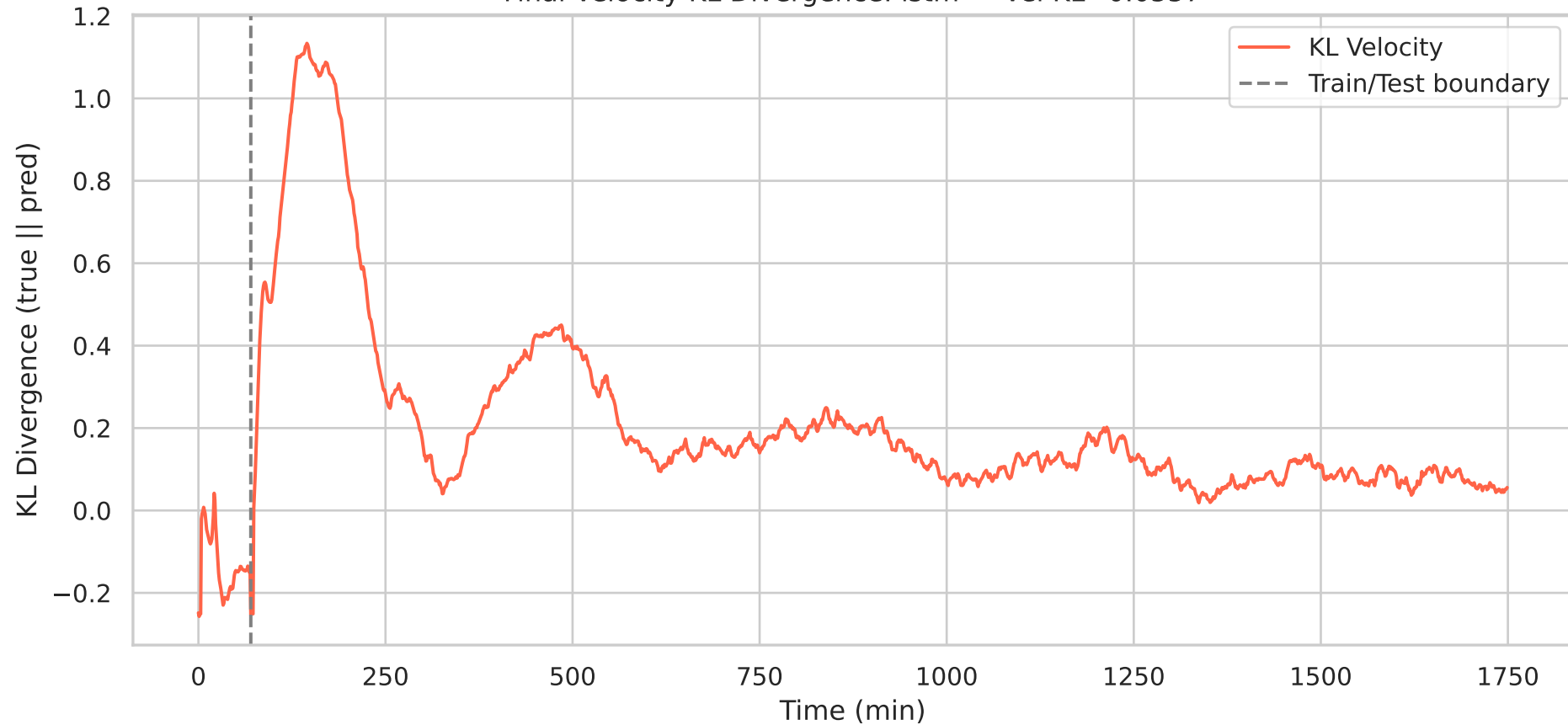
Final Velocity KL Divergence: lstm — Vel KL=0.0557
