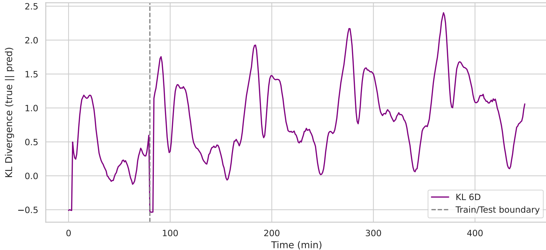
Full 6D KL Divergence: Istm — KL=1.0593
