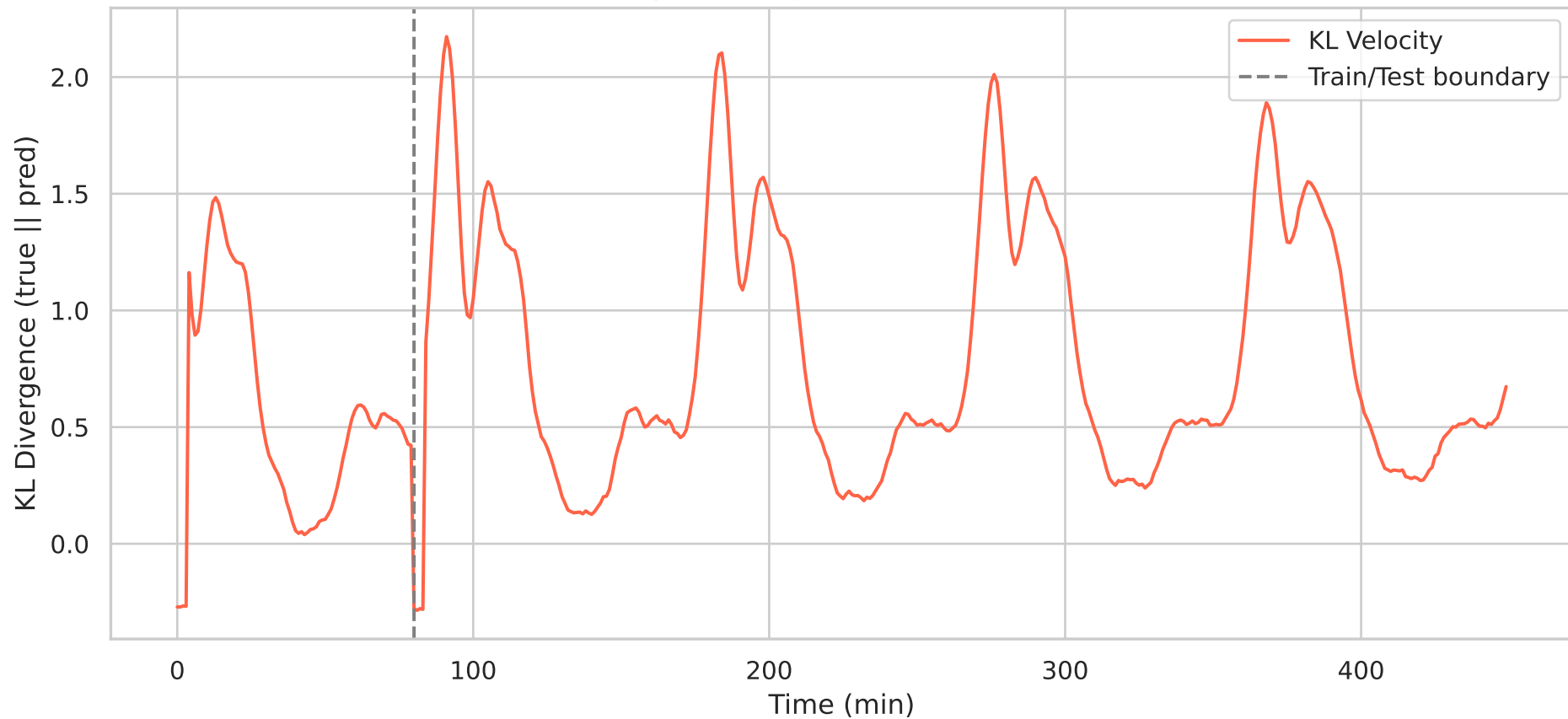
Final Velocity KL Divergence: lstm — Vel KL=0.6735
