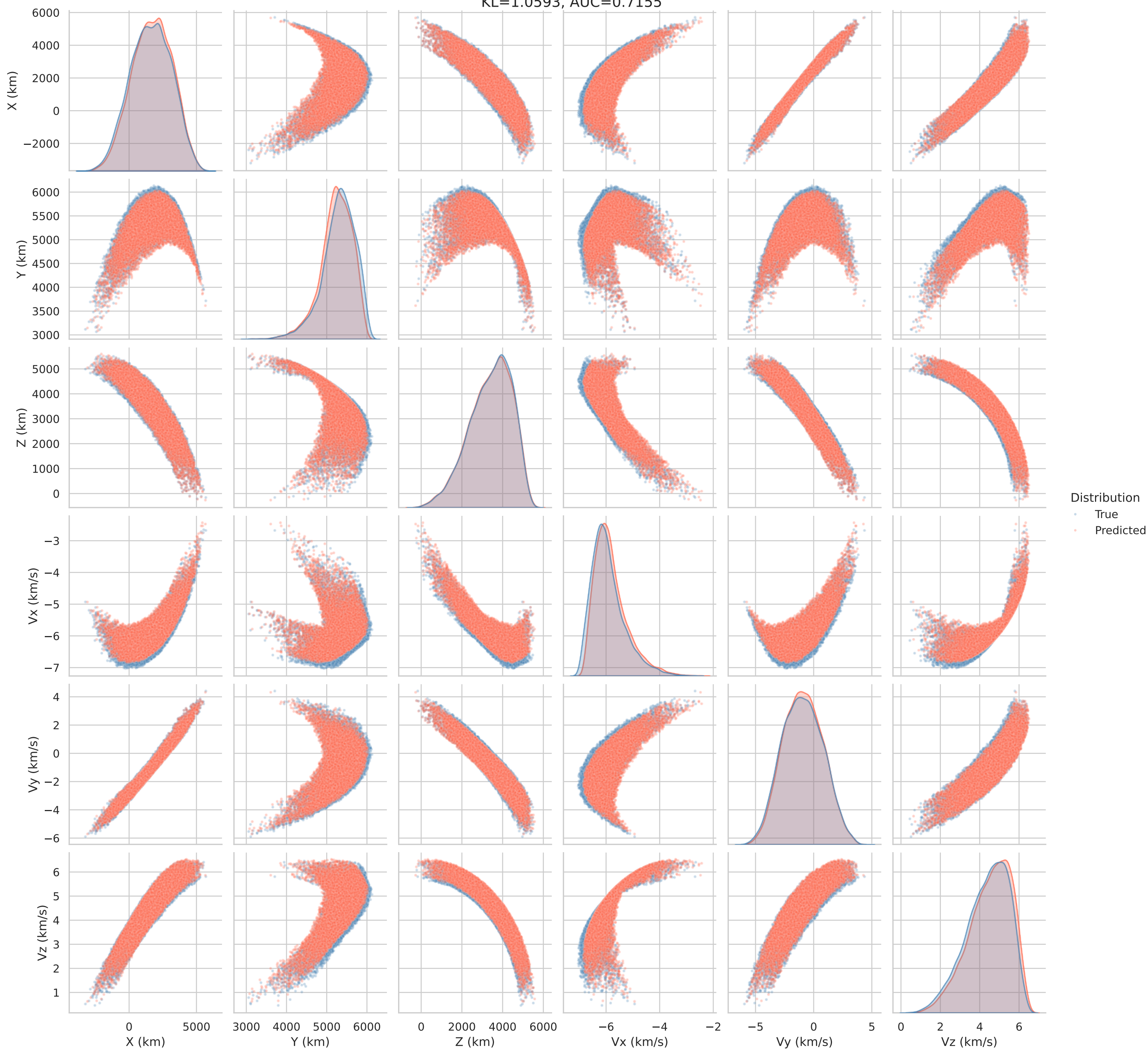
Istm Final State Pairplot — True vs Predicted KL=1.0593, AUC=0.7155
