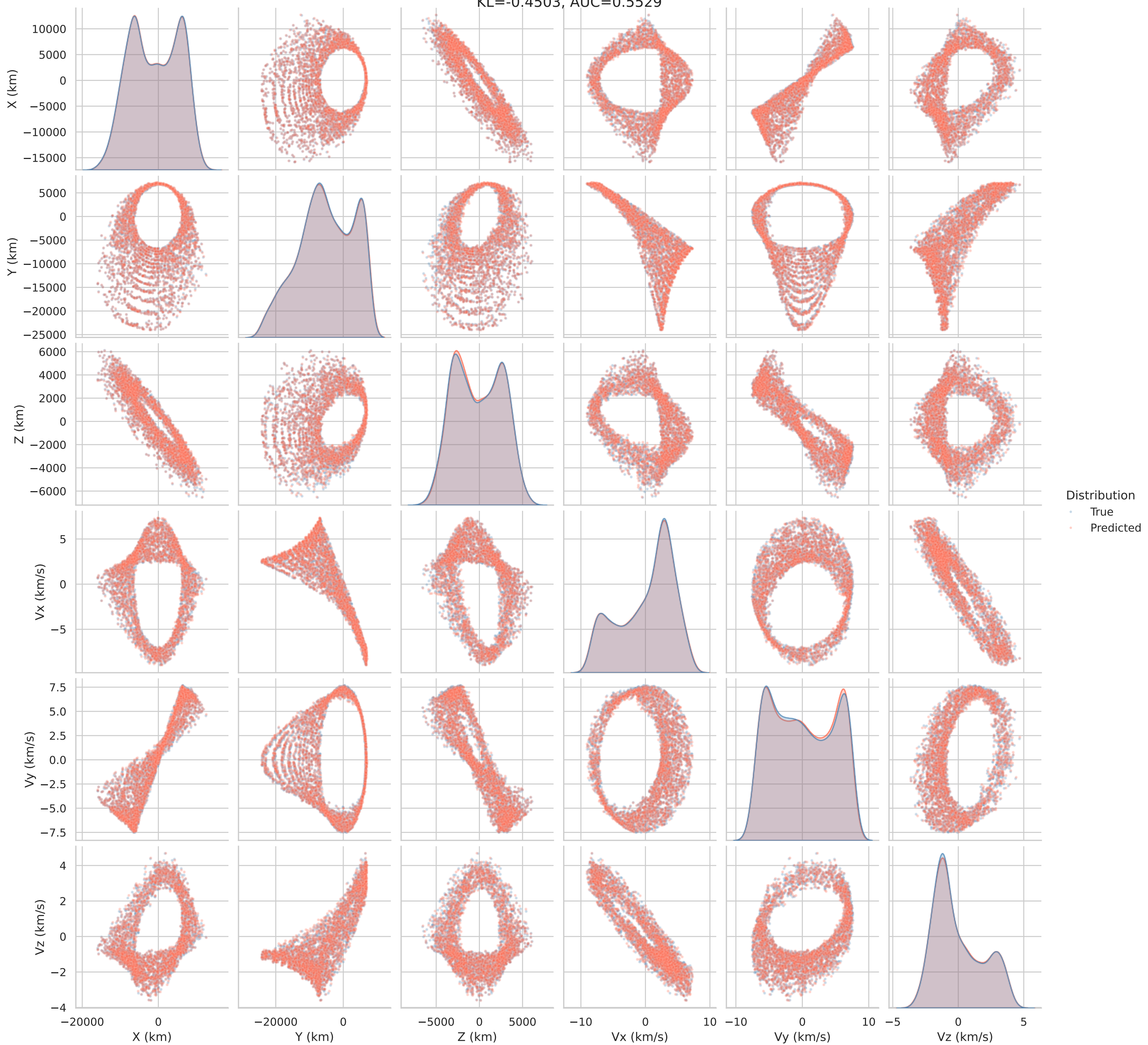
mamba Final State Pairplot — True vs Predicted KL=-0.4503, AUC=0.5529
