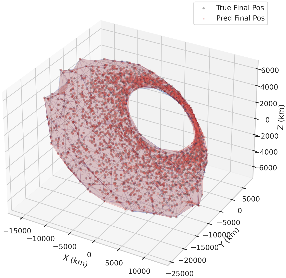
mamba Final State Positions Alpha Shape Vol Ratio (Pred/True): 1.0063
