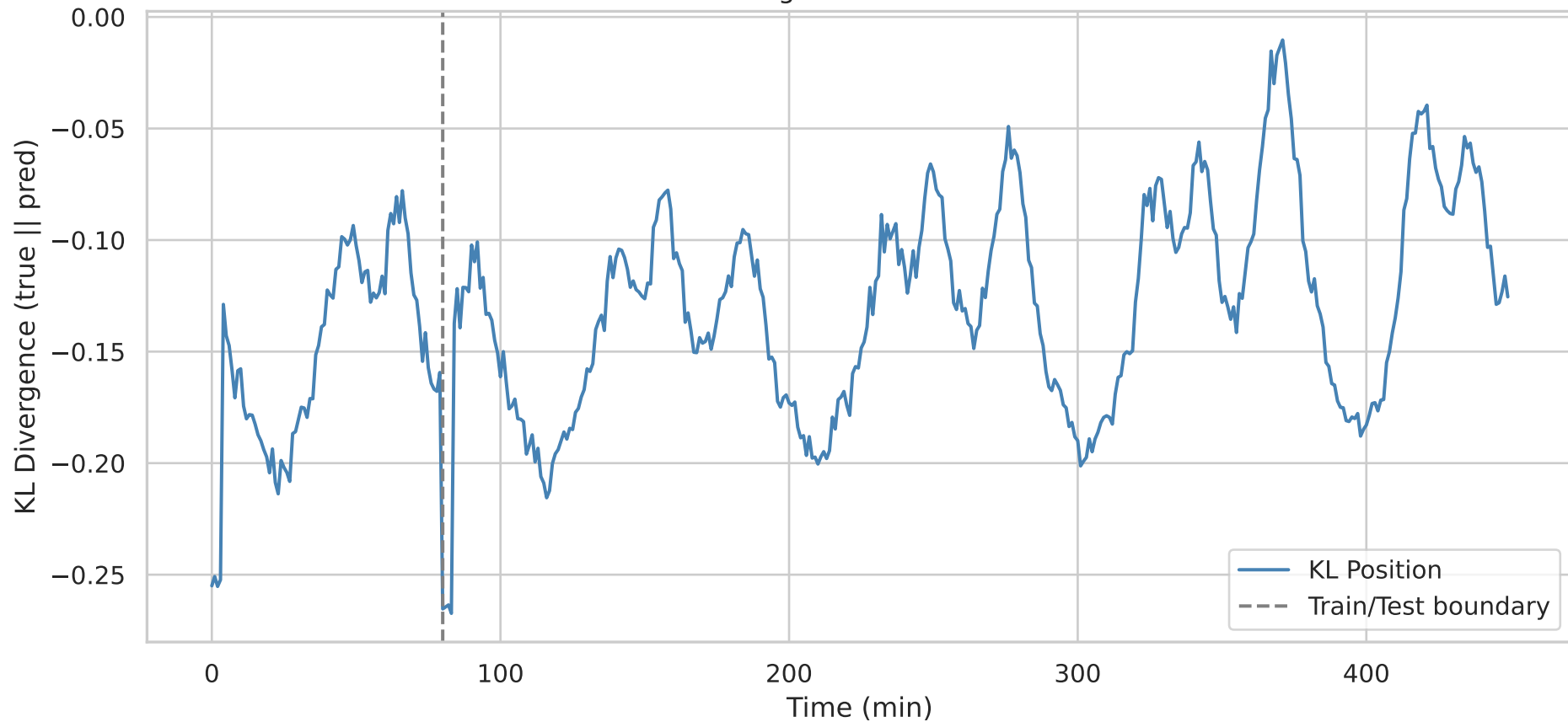
Final Position KL Divergence: mamba — Pos KL=-0.1255
