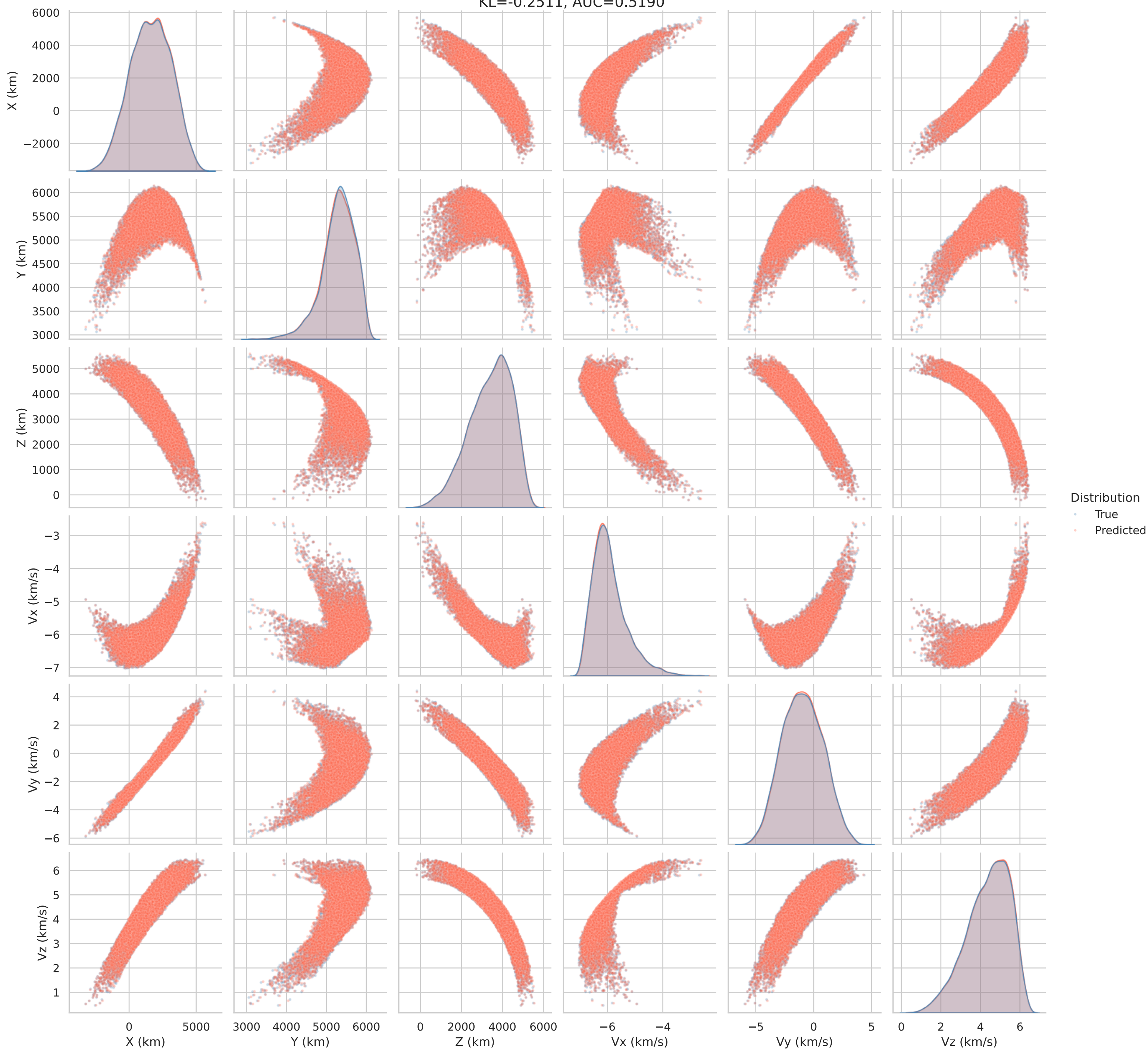
mamba Final State Pairplot — True vs Predicted KL=-0.2511, AUC=0.5190
