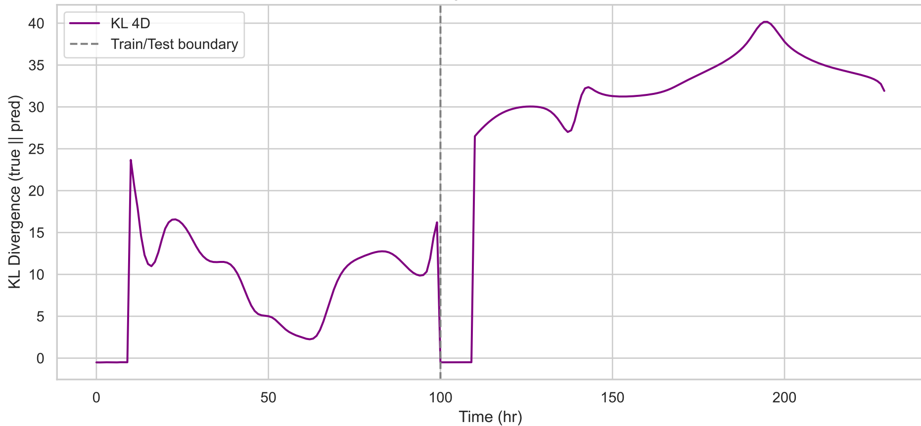
Full 4D KL Divergence: Istm — KL=31.9124
