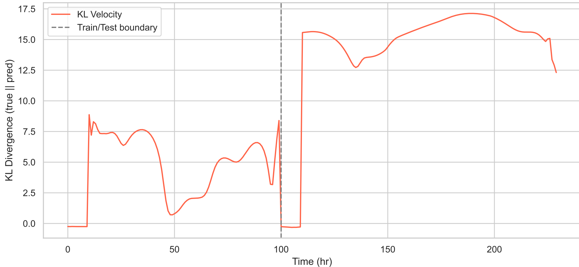
Final Velocity KL Divergence: Istm — Vel KL=12.3099
