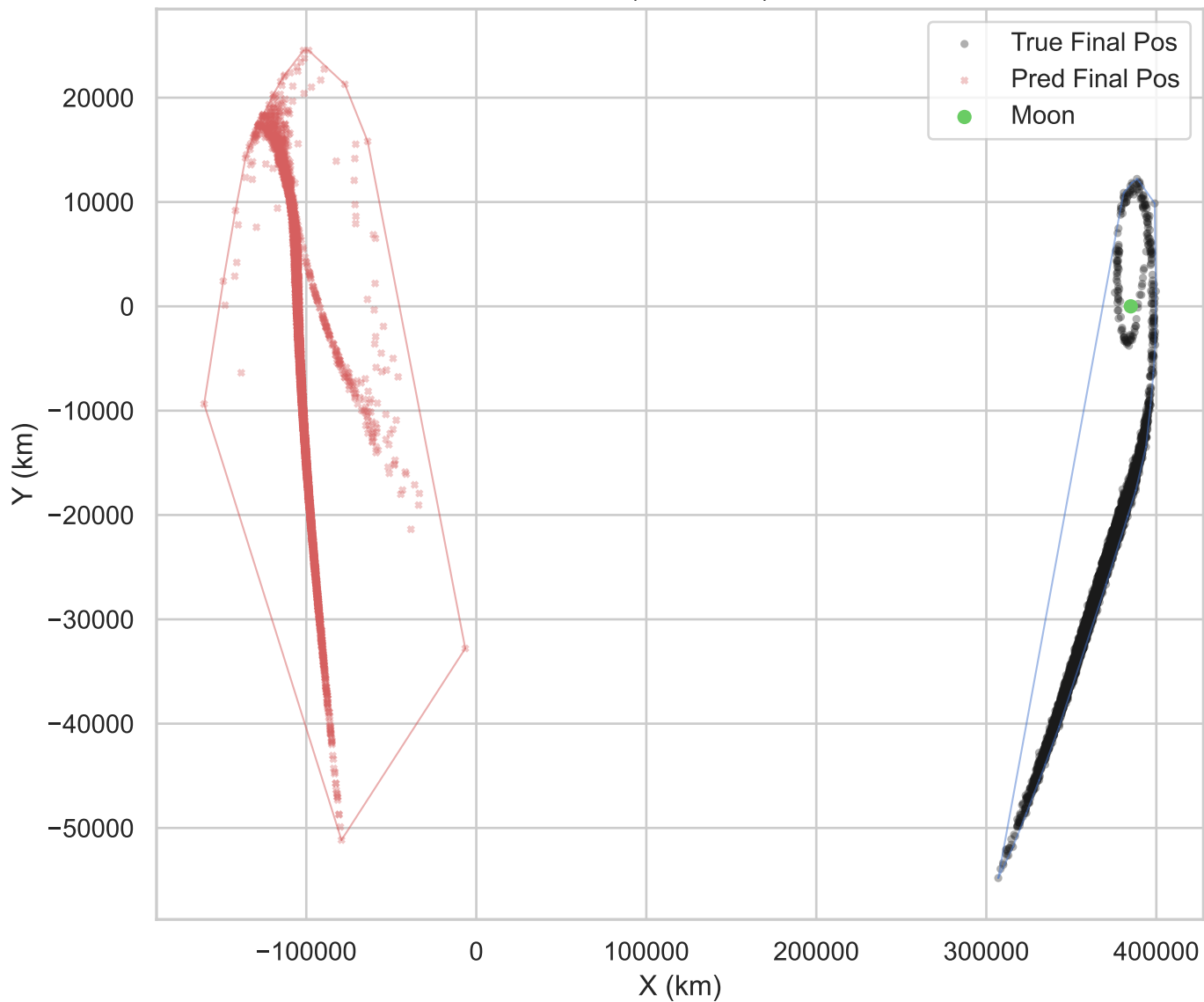
Istm Final State Positions Convex Hull Area Ratio (Pred/True): 3.7352
