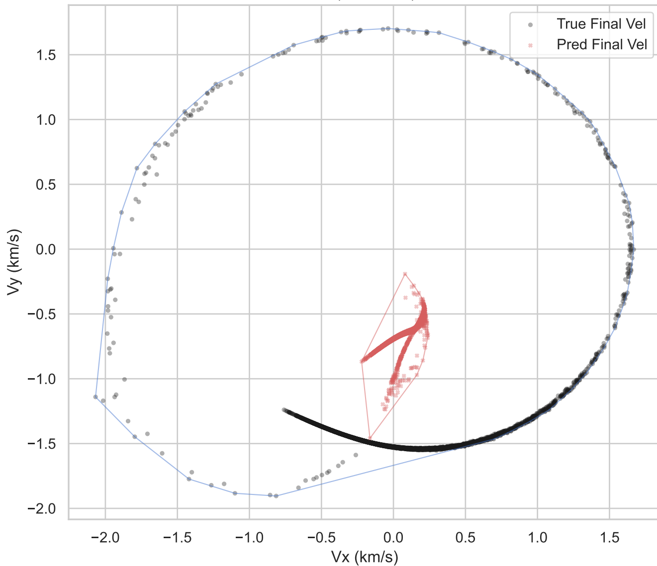
Istm Final State Velocities Convex Hull Area Ratio (Pred/True): 0.0306
