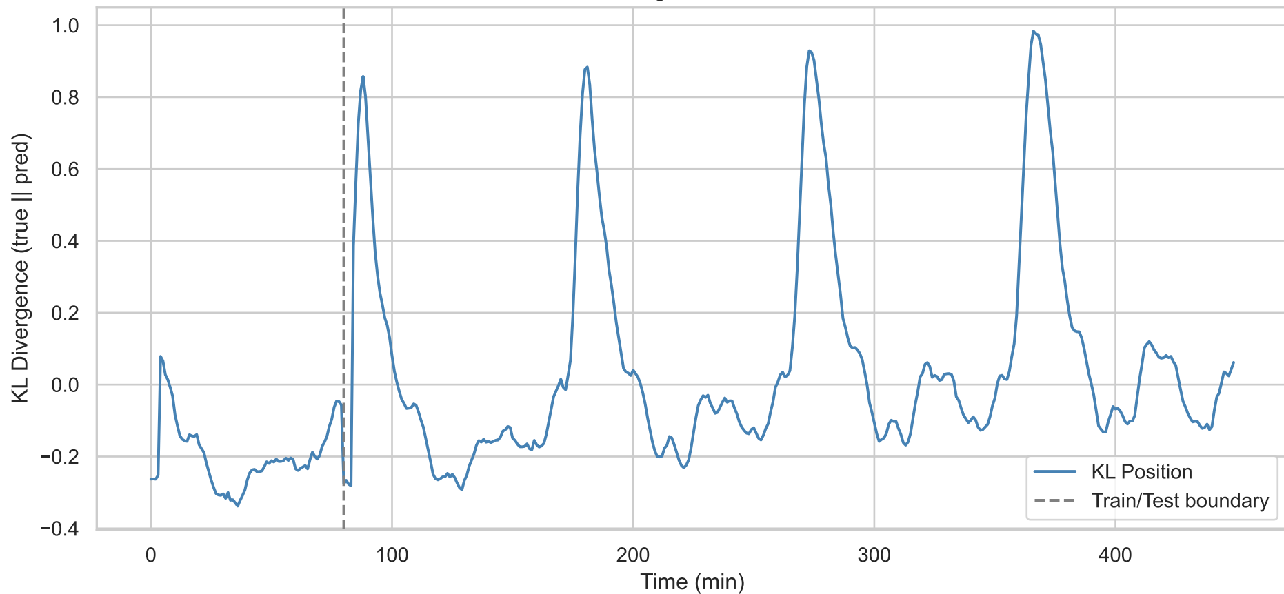
Final Position KL Divergence: lstm — Pos KL=0.0618
