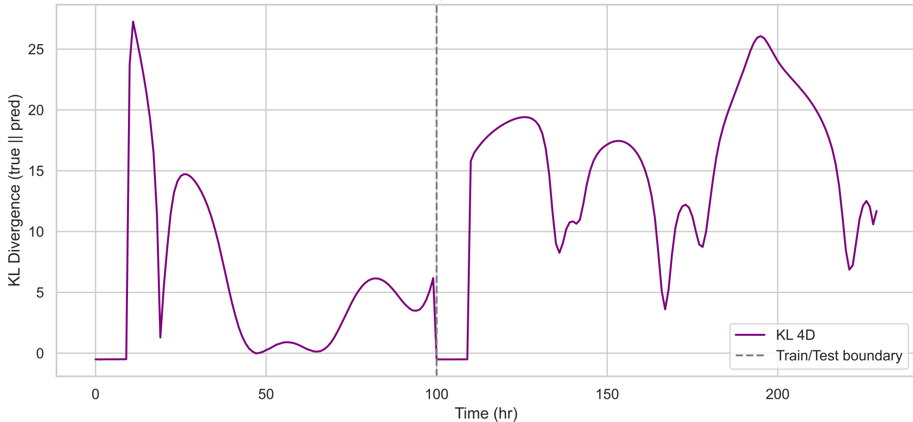
Full 4D KL Divergence: mamba — KL=11.6957
