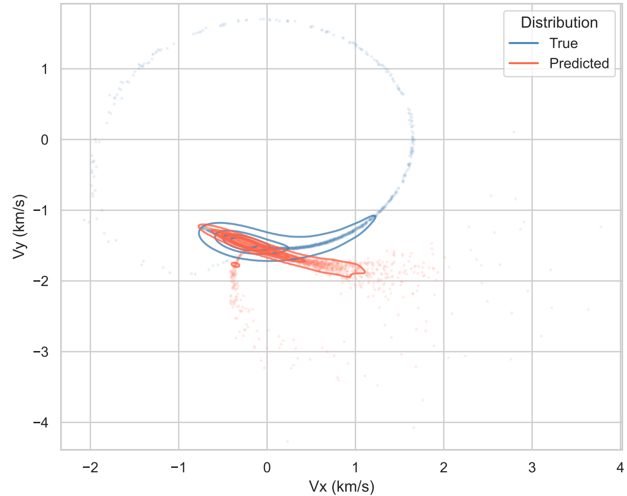
Final State PDF: mamba
