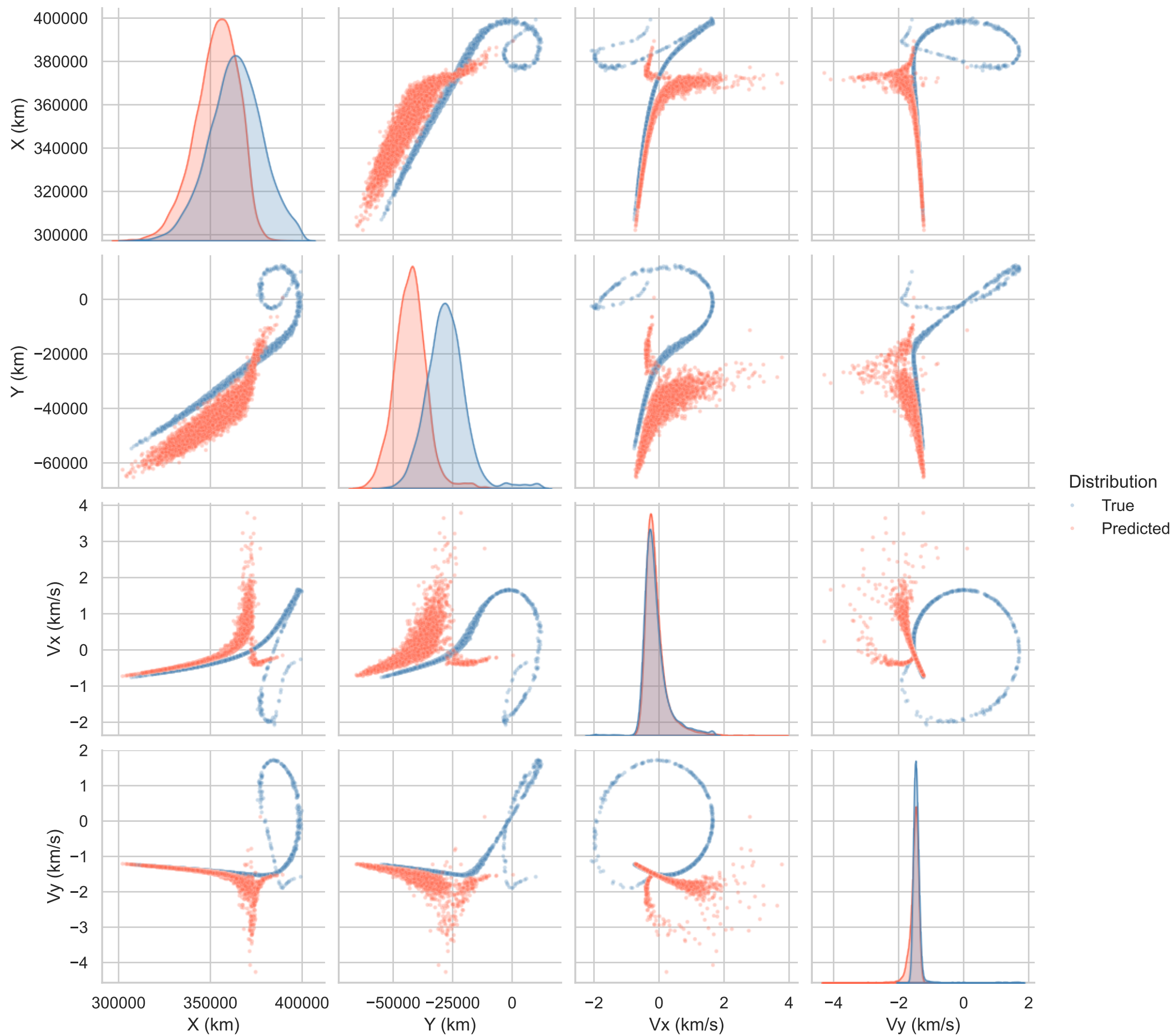
mamba Final State Pairplot — True vs Predicted
