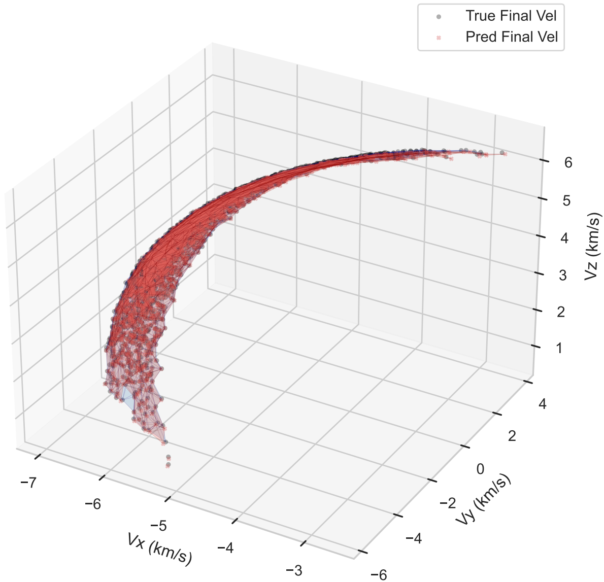
mamba Final State Velocities Alpha Shape Vol Ratio (Pred/True): 1.4756
