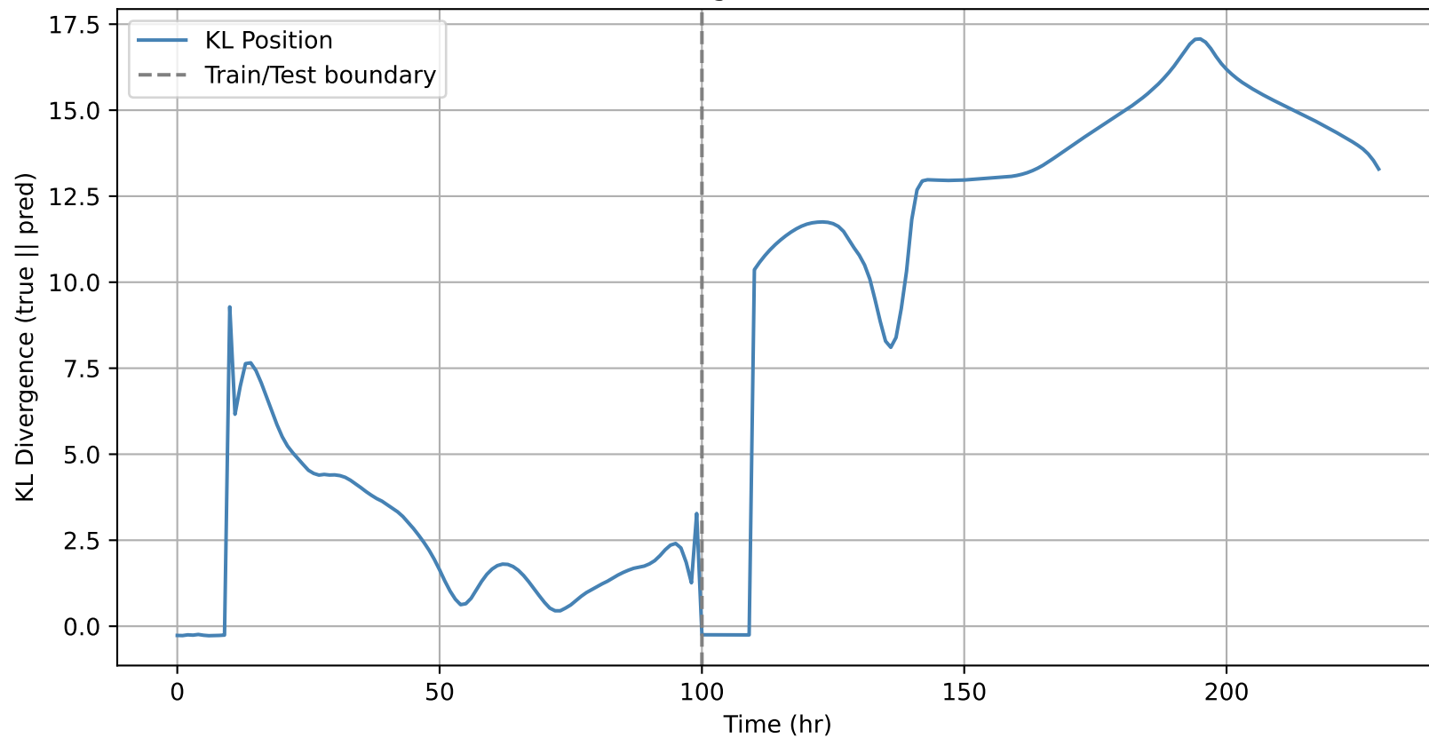
Final Position KL Divergence: lstm — Pos KL=13.2896
