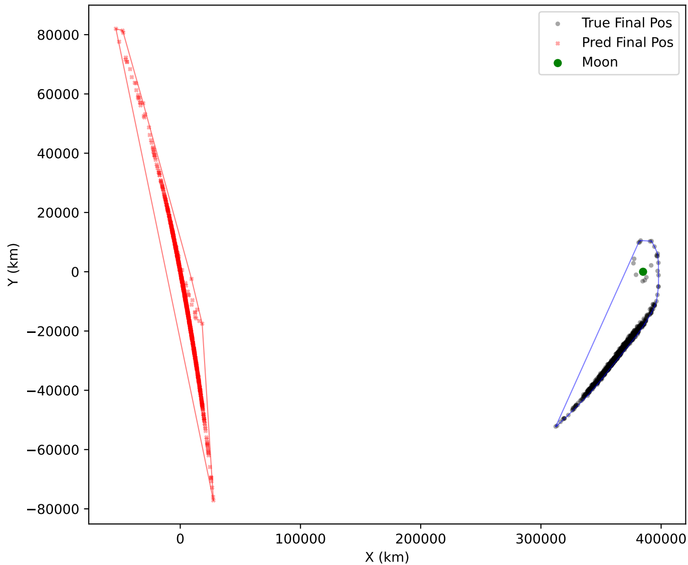
Istm Final-State Positions Convex Hull Area Ratio (Pred/True): 1.3163
