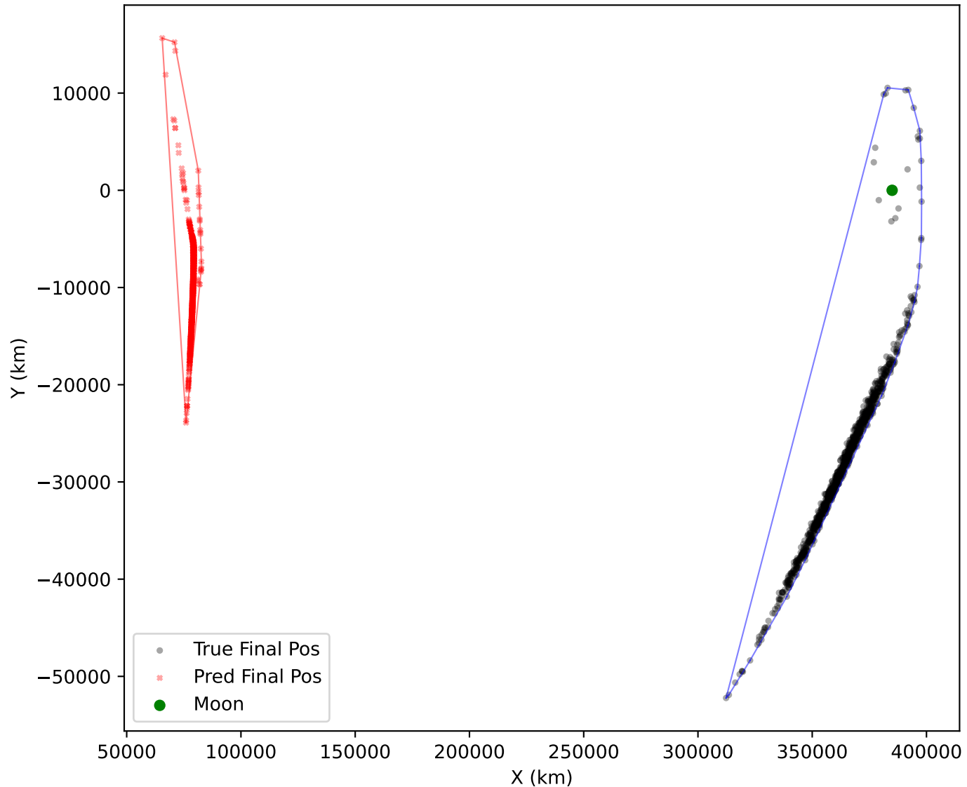
Istm Final-State Positions Convex Hull Area Ratio (Pred/True): 0.2098
