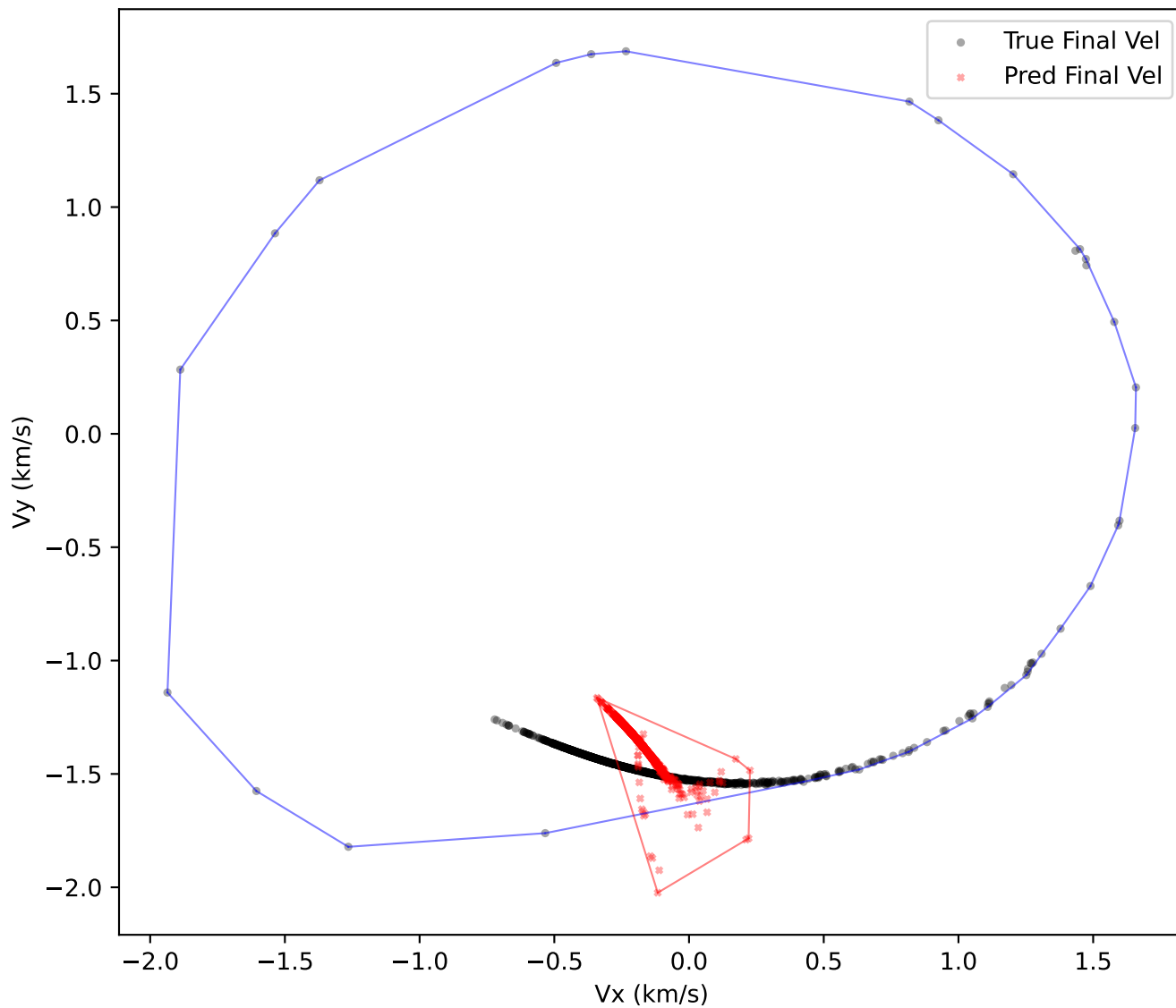
Istm Final-State Velocities Convex Hull Area Ratio (Pred/True): 0.0268
