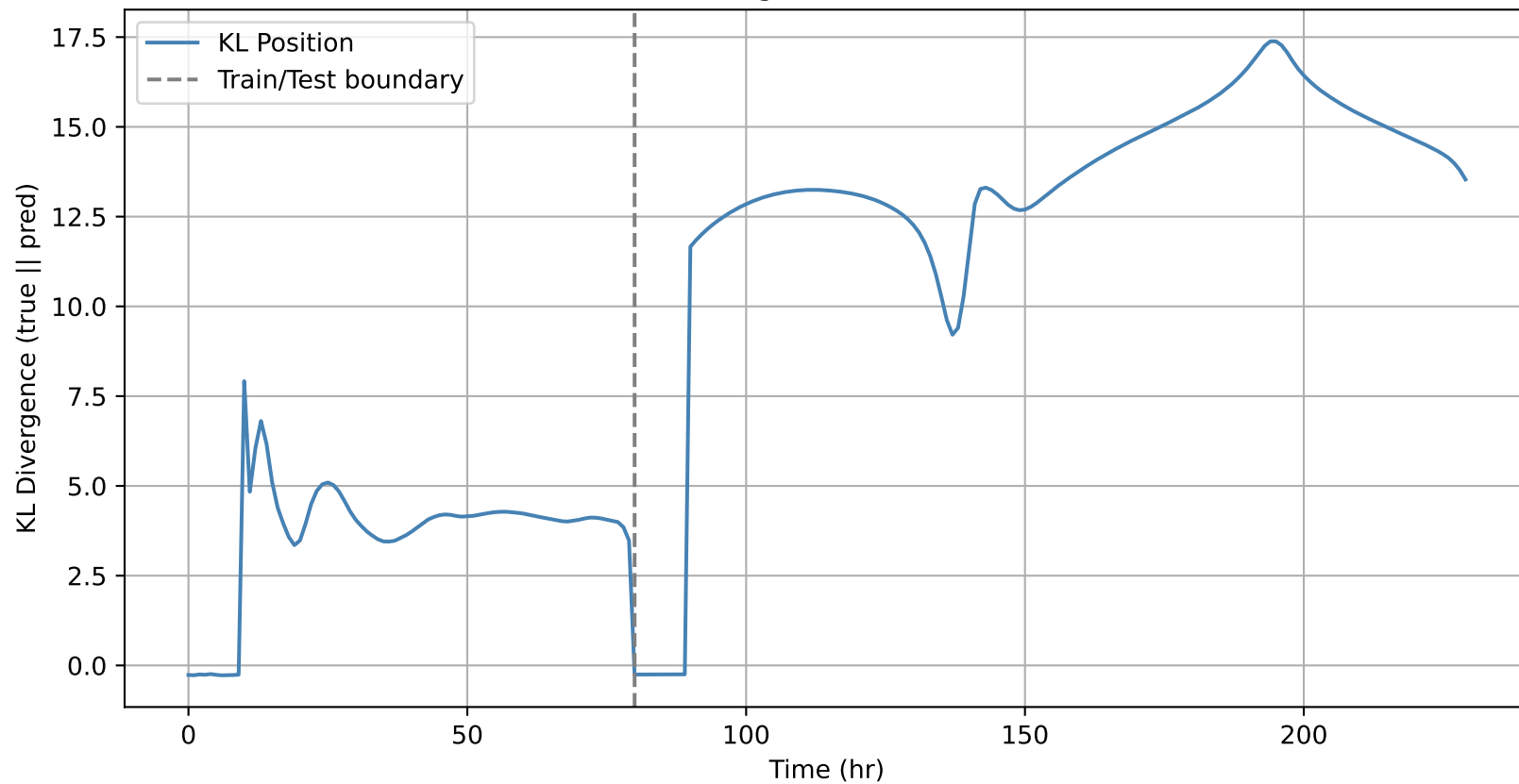
Final Position KL Divergence: lstm — Pos KL=13.5347
