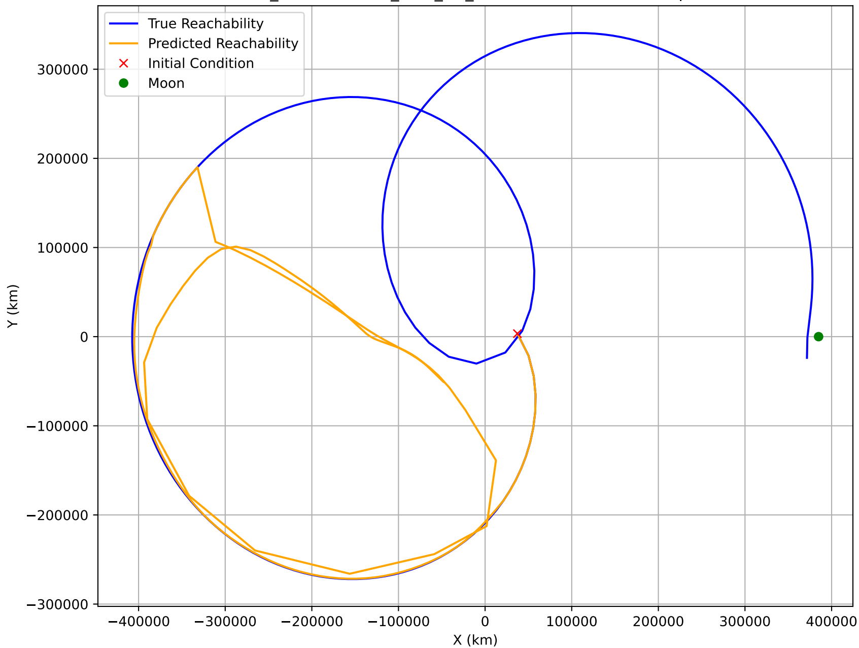
LSTM Reachability Prediction for Trajectory 124 Orbit: 2.1_RETROGRADE_GEO_TO_MOON, Train Ratio: 0.1, Epochs: 10
