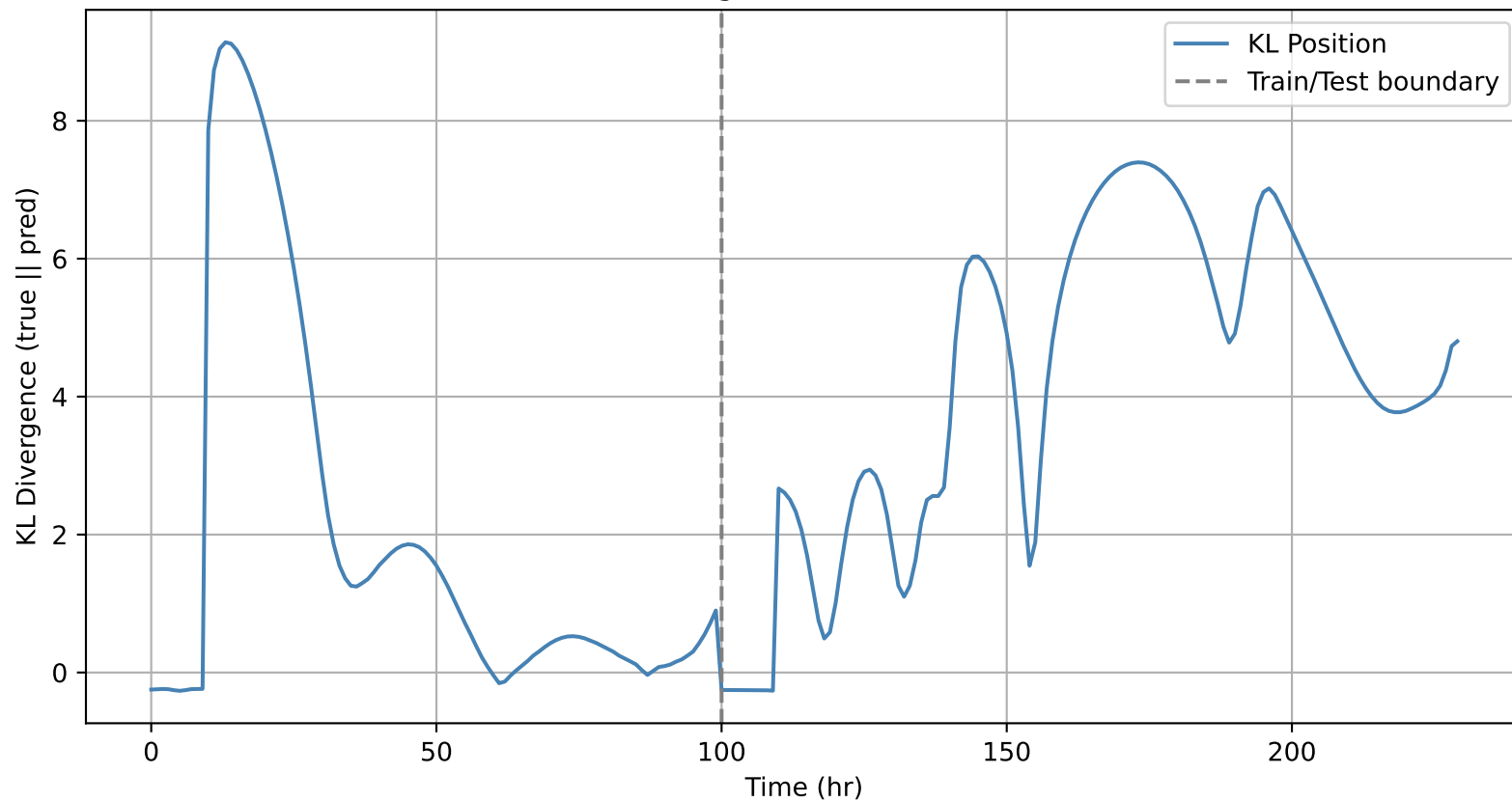
Final Position KL Divergence: mamba — Pos KL=4.8025
