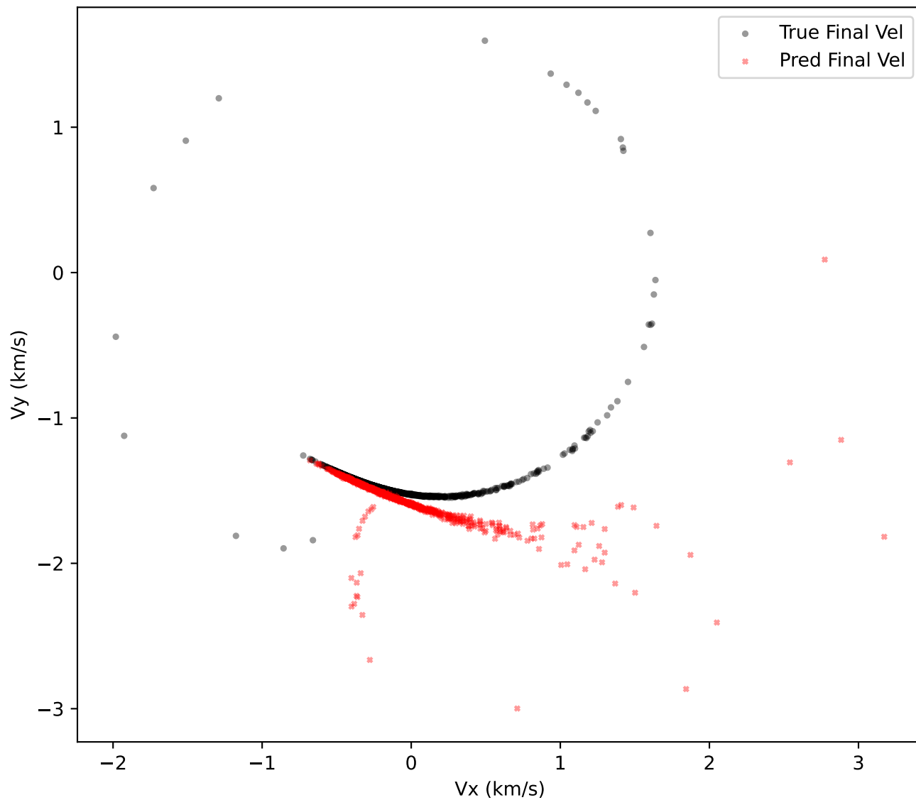
mamba Final-State Velocities
