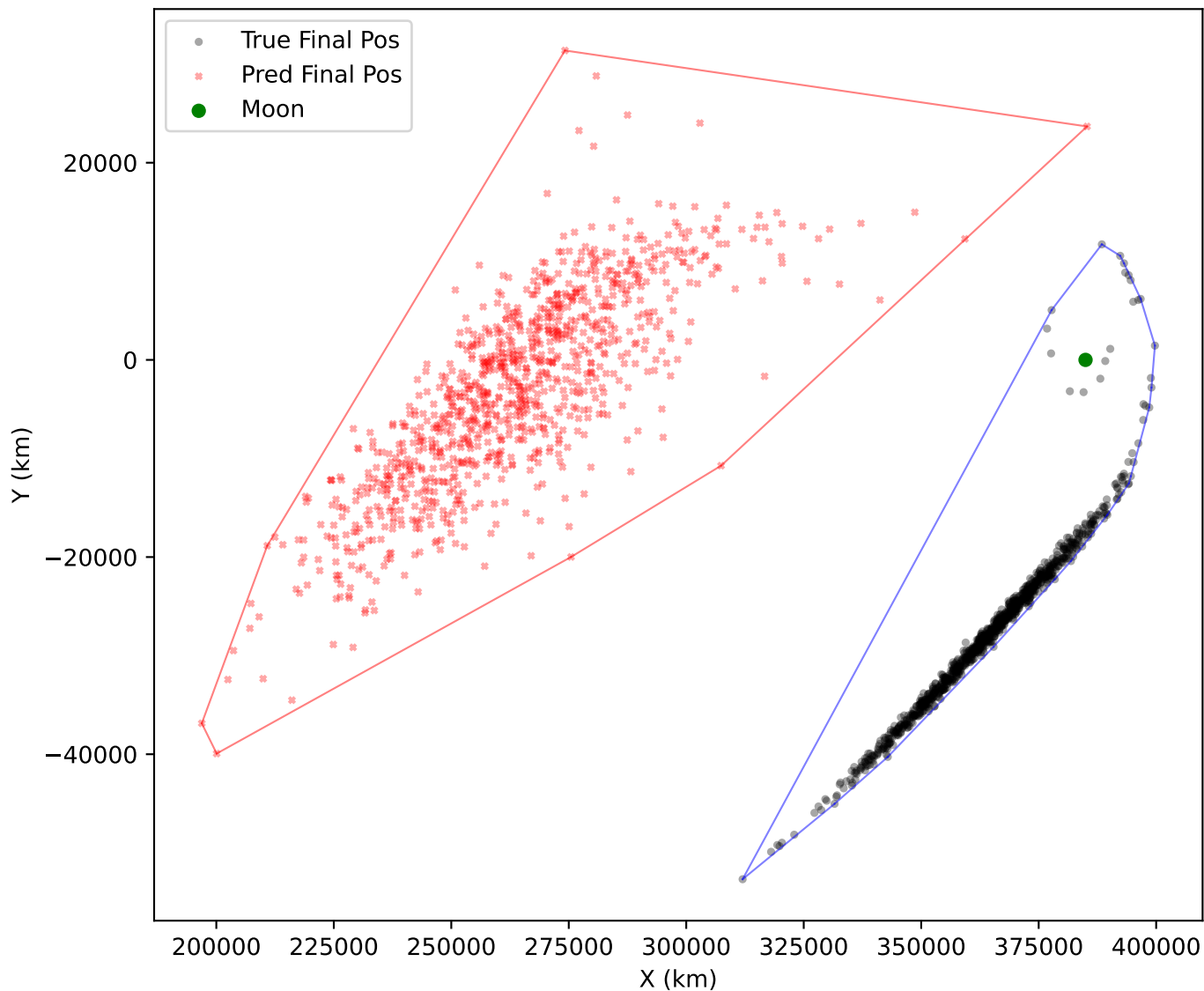
mamba Final-State Positions Convex Hull Area Ratio (Pred/True): 3.6532
