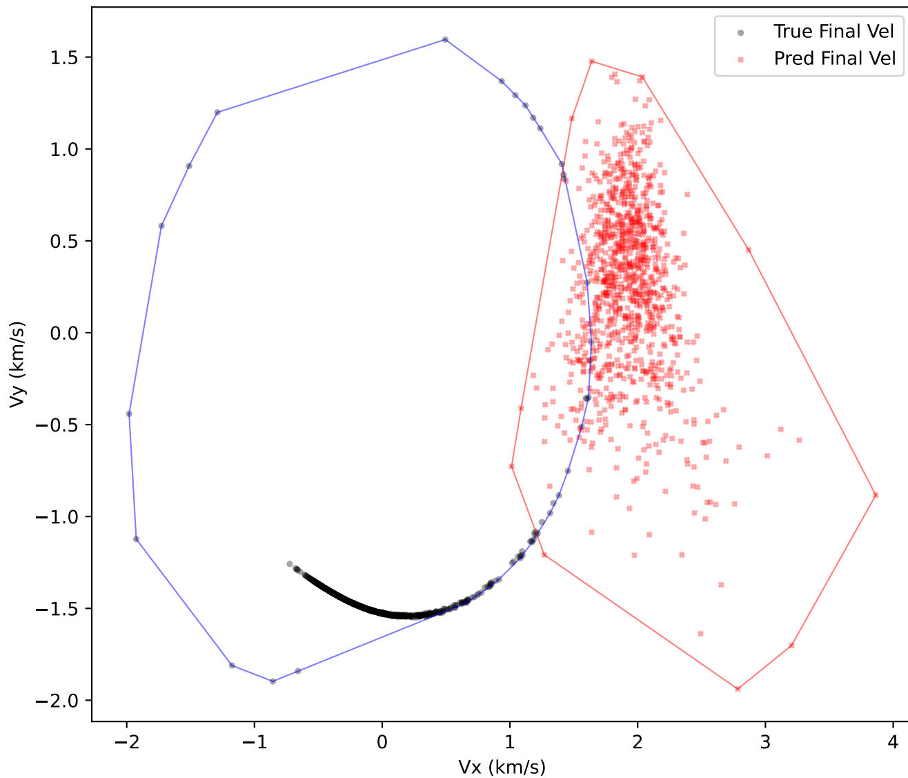
mamba Final-State Velocities Convex Hull Area Ratio (Pred/True): 0.5940
