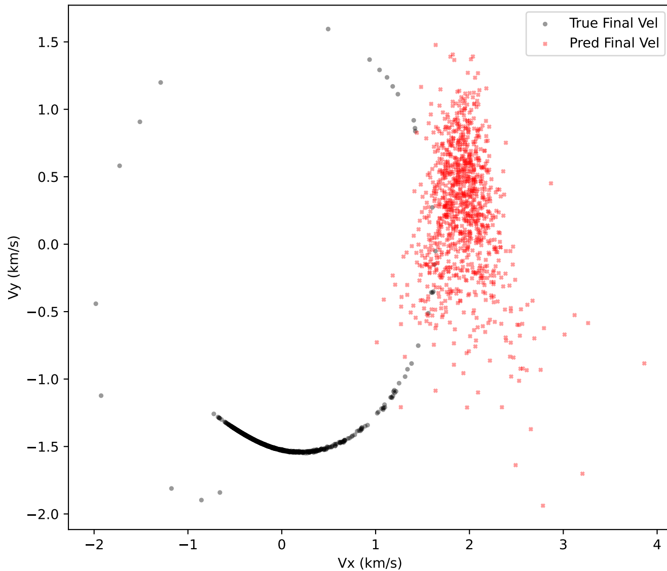
mamba Final-State Velocities
