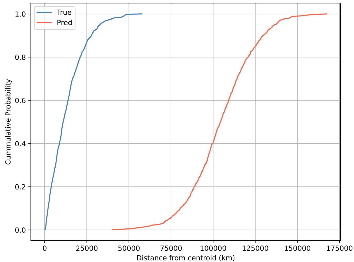
Position CDF
