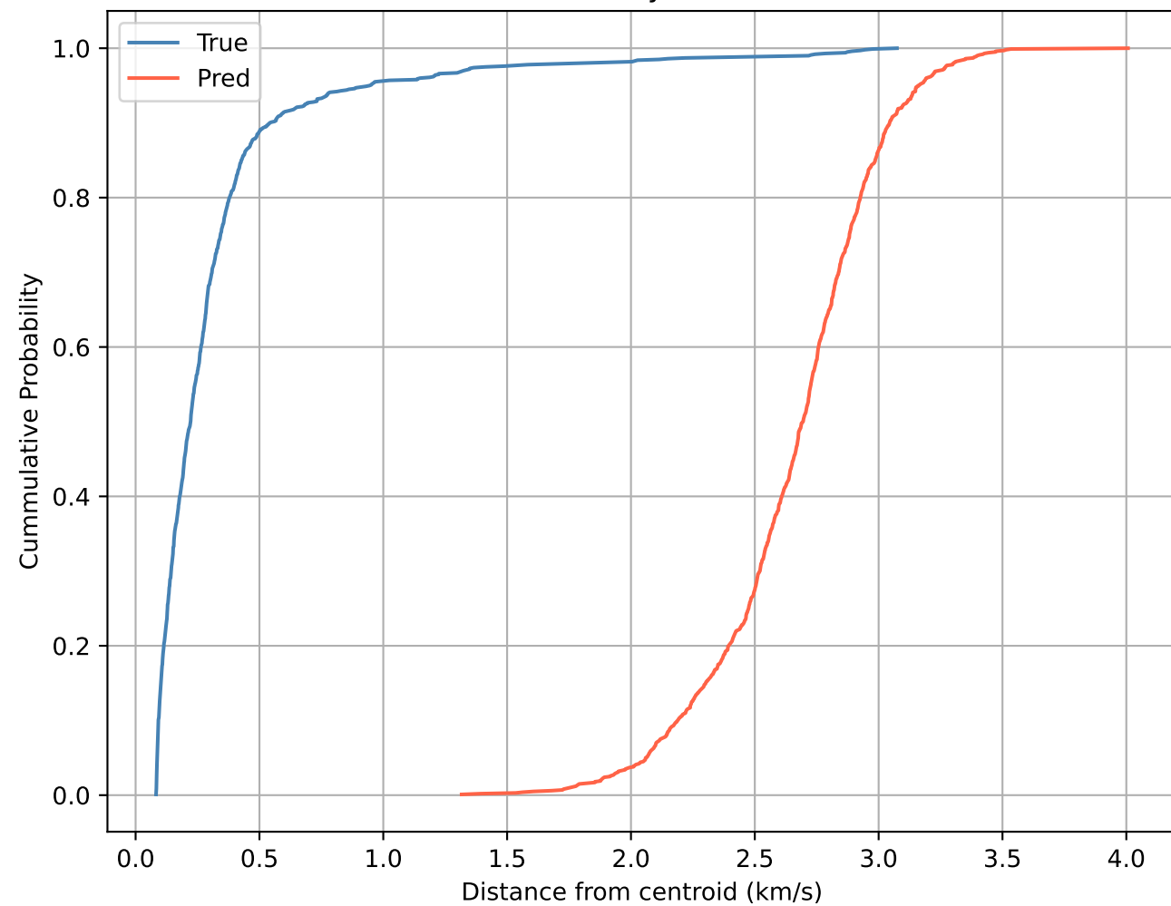
Velocity CDF
