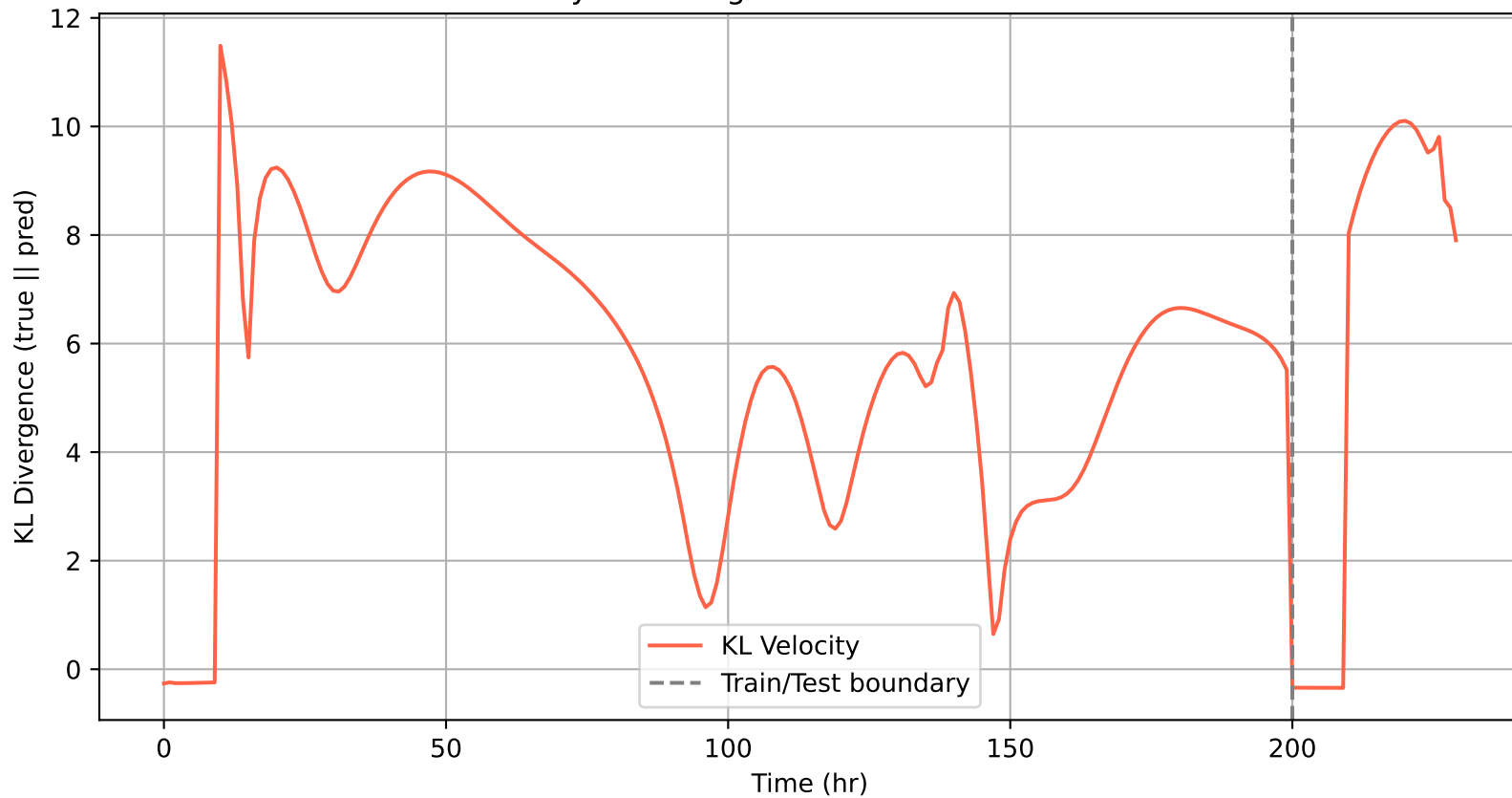
Final Velocity KL Divergence: mamba — Vel KL=7.9028
