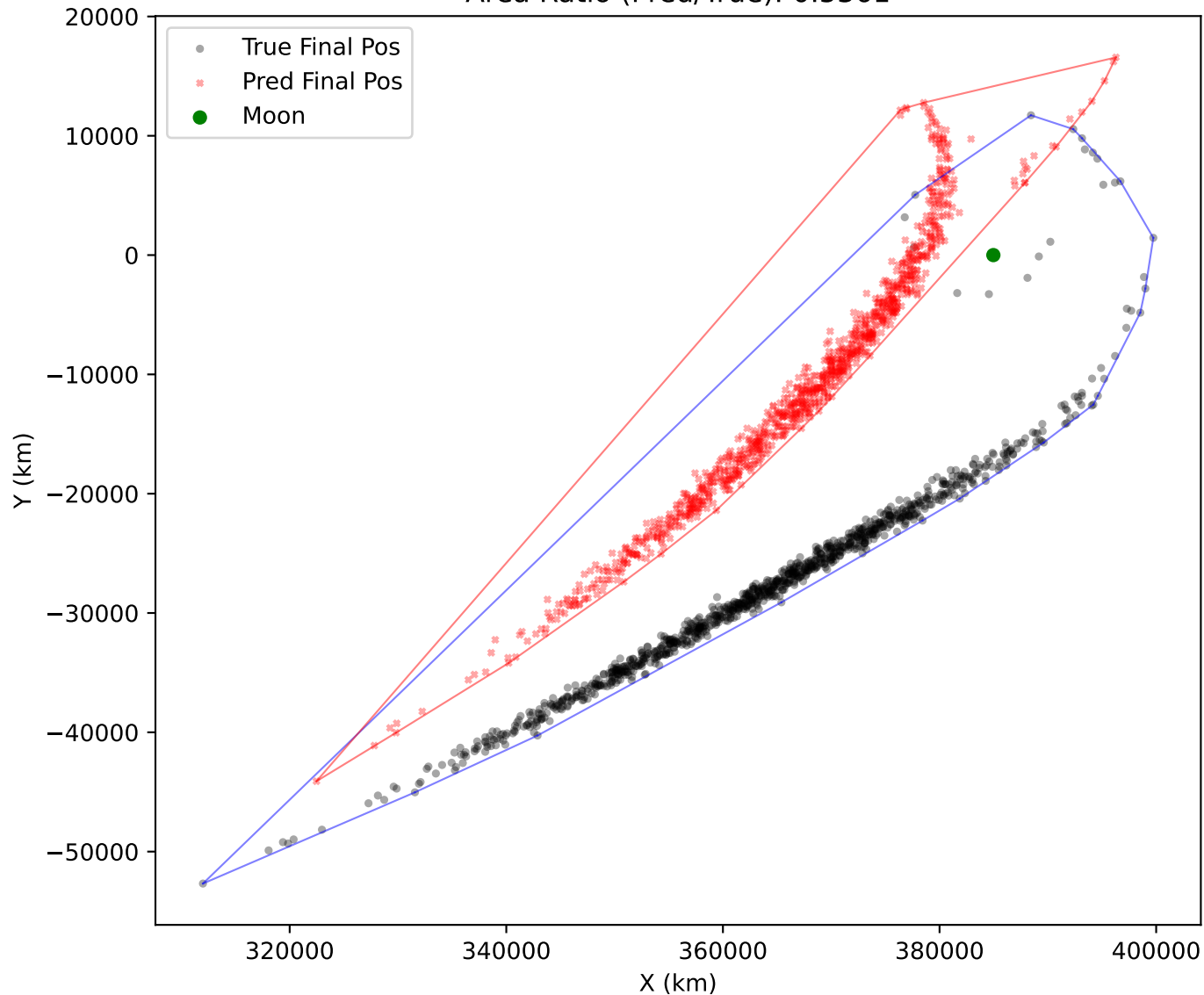
mamba Final-State Positions Convex Hull Area Ratio (Pred/True): 0.5361
