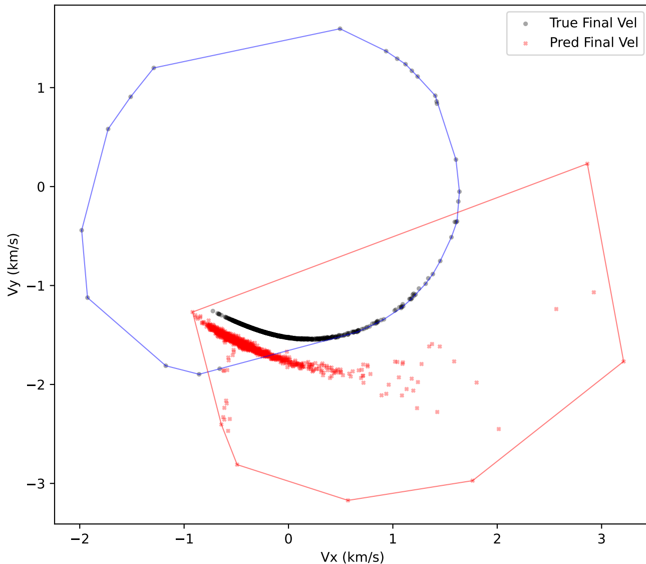
mamba Final-State Velocities Convex Hull Area Ratio (Pred/True): 0.9348
