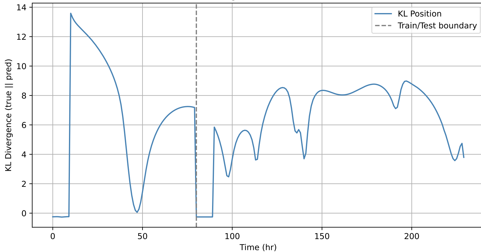
Final Position KL Divergence: mamba — Pos KL=3.7918
