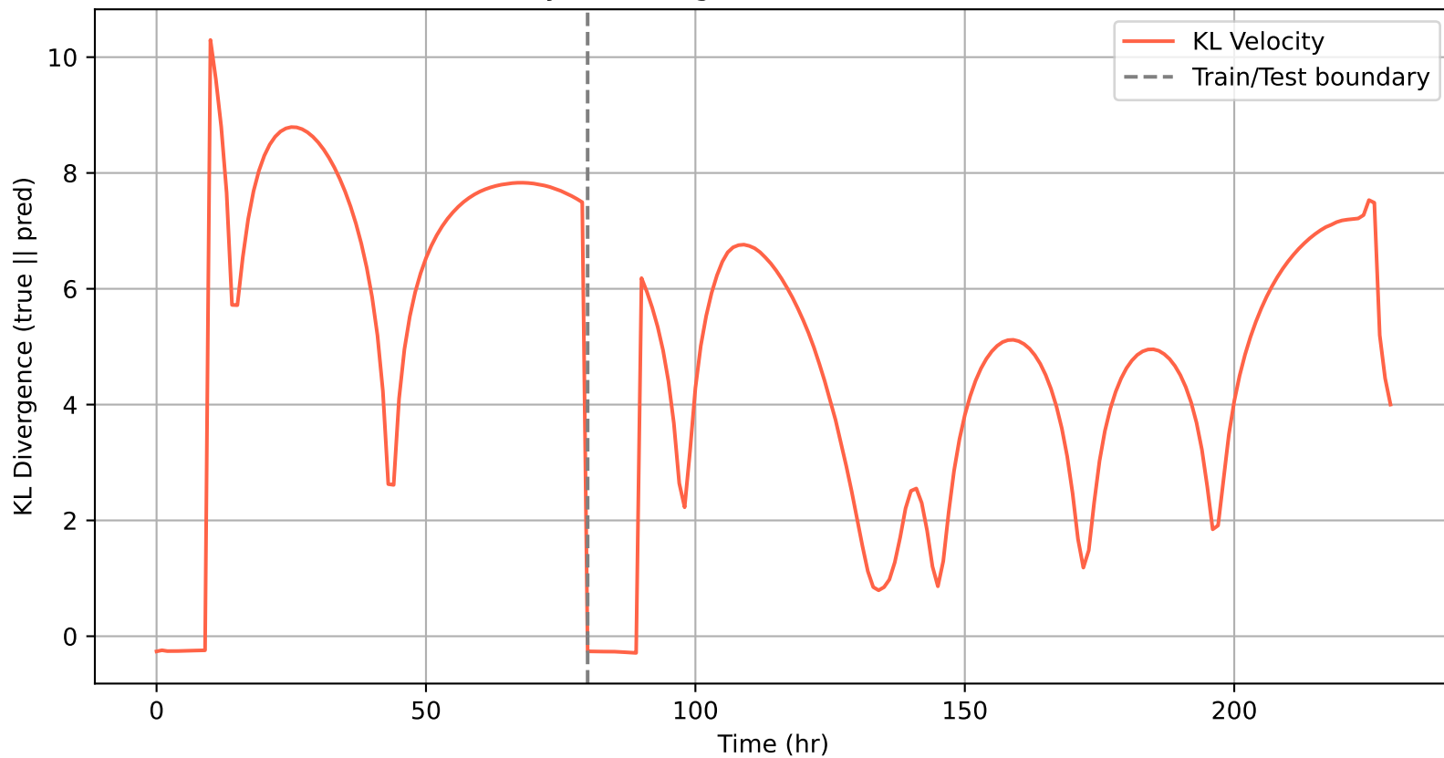
Final Velocity KL Divergence: mamba — Vel KL=4.0004
