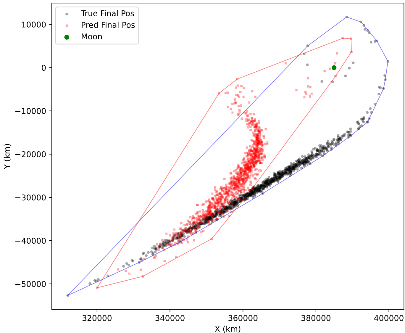
mamba Final-State Positions Convex Hull Area Ratio (Pred/True): 0.8529
