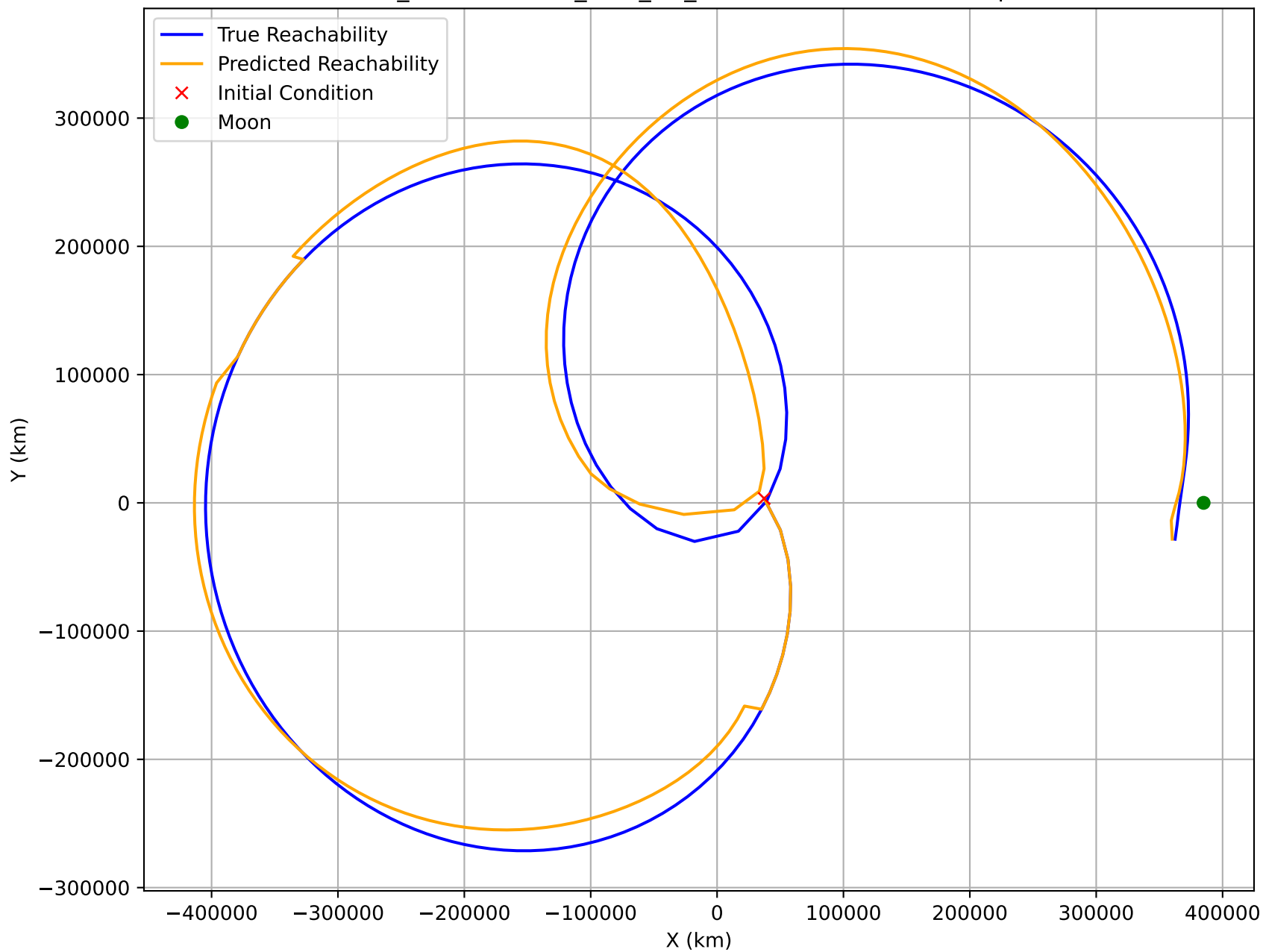
MAMBA Reachability Prediction for Trajectory 124 Orbit: 2.1_RETROGRADE_GEO_TO_MOON, Train Ratio: 0.1, Epochs: 10
