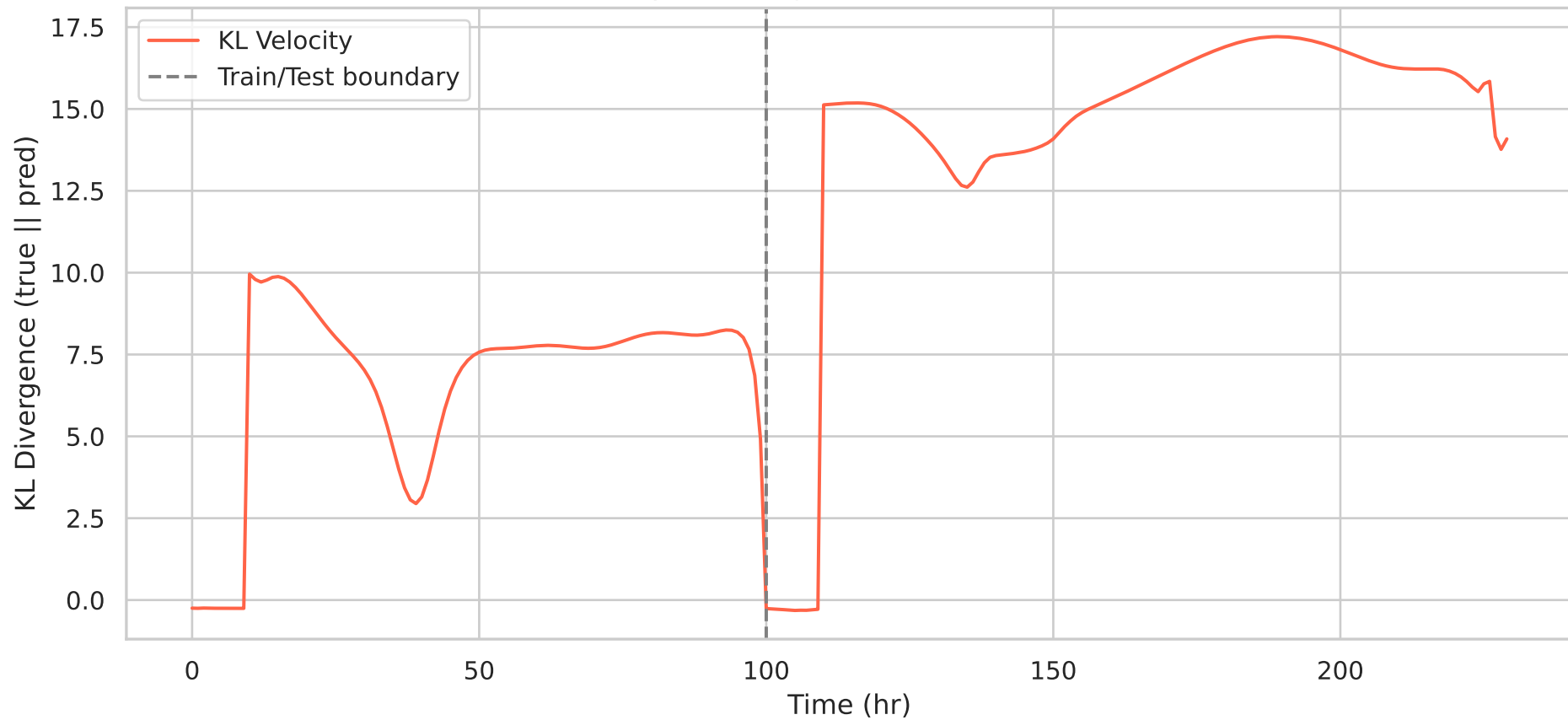
Final Velocity KL Divergence: lstm — Vel KL=14.0852
