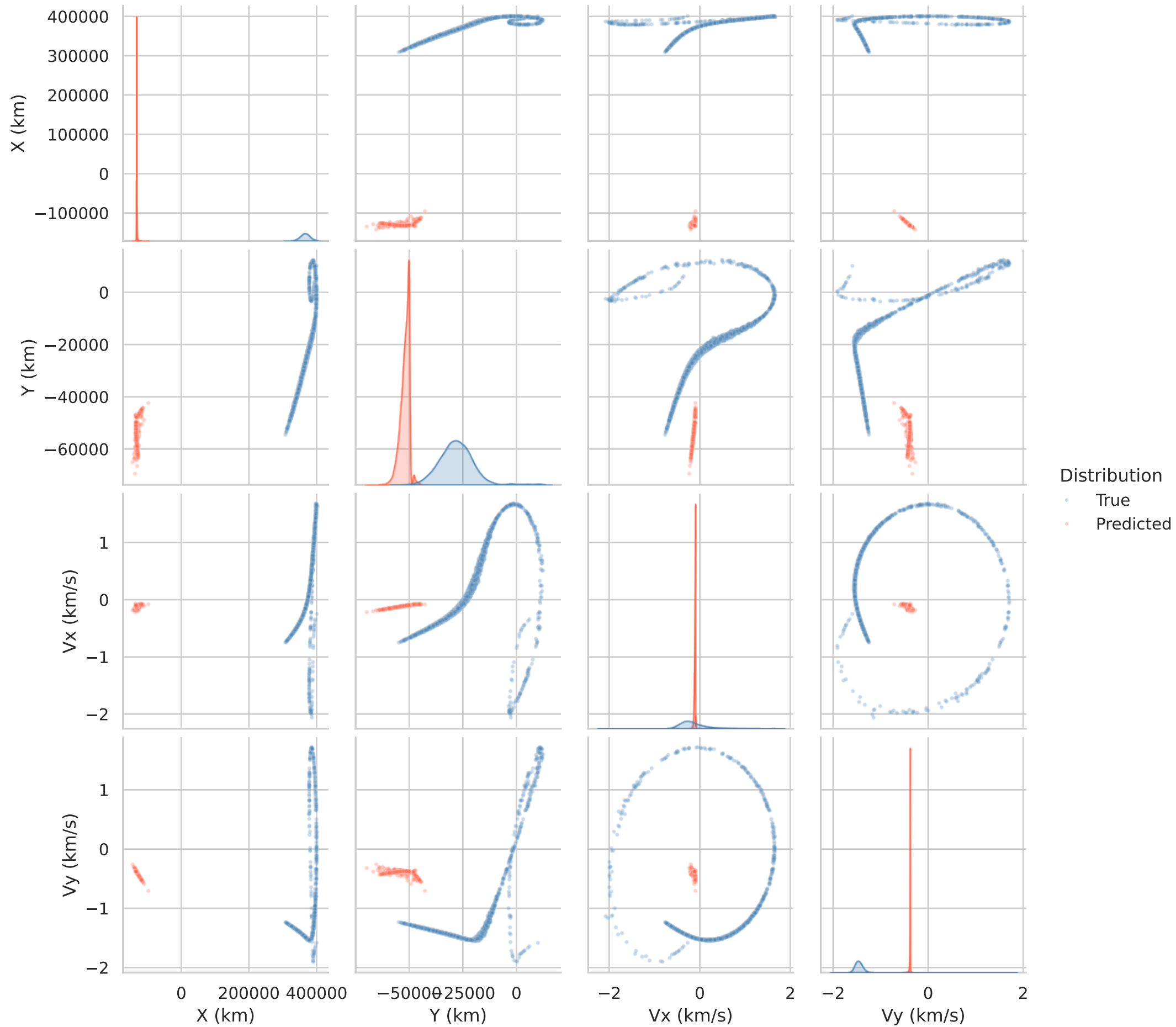
Istm Final State Pairplot — True vs Predicted
