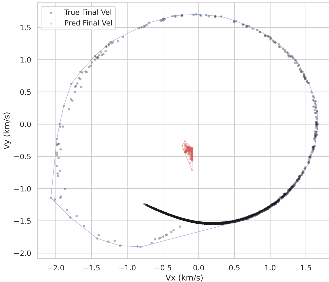
Istm Final State Velocities Convex Hull Area Ratio (Pred/True): 0.0030
