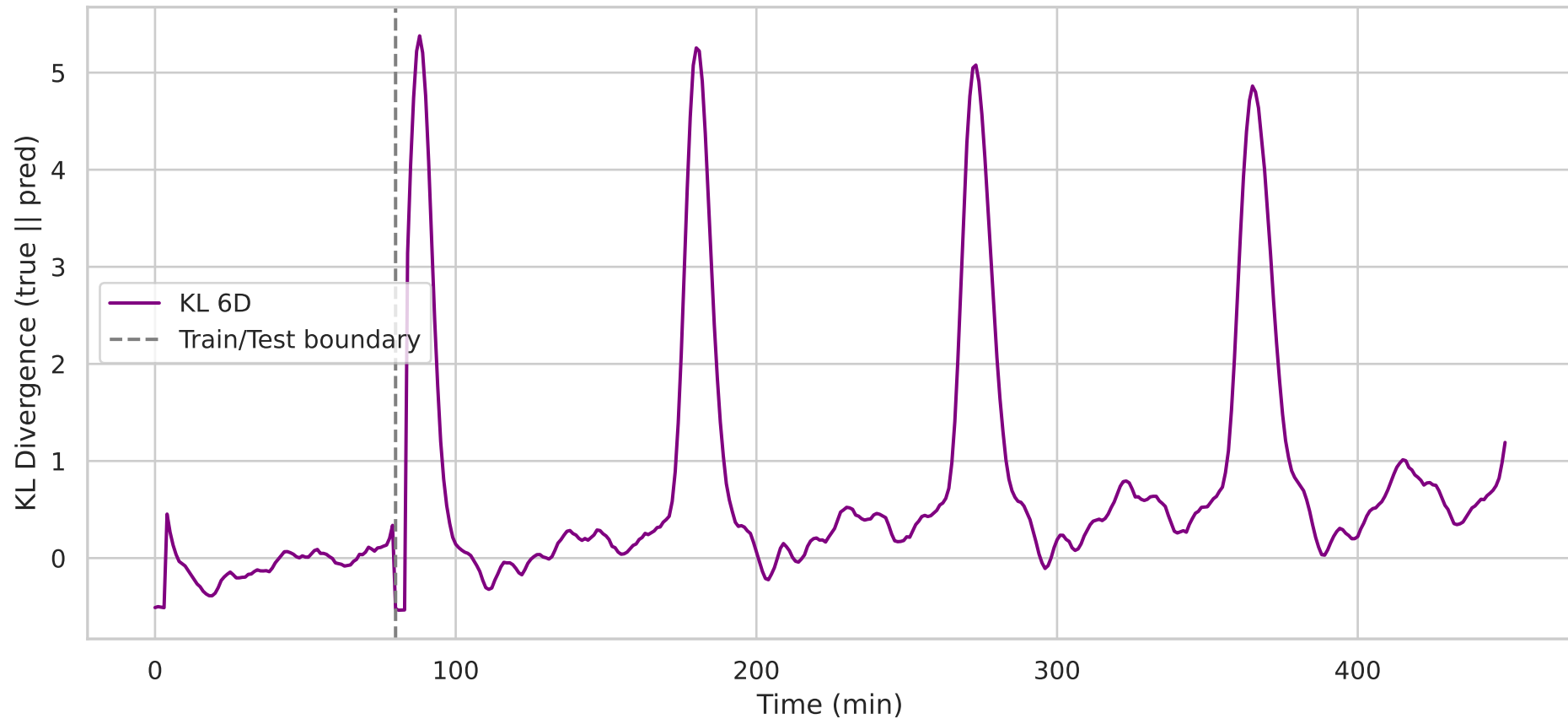
Full 6D KL Divergence: lstm — KL=1.1912
