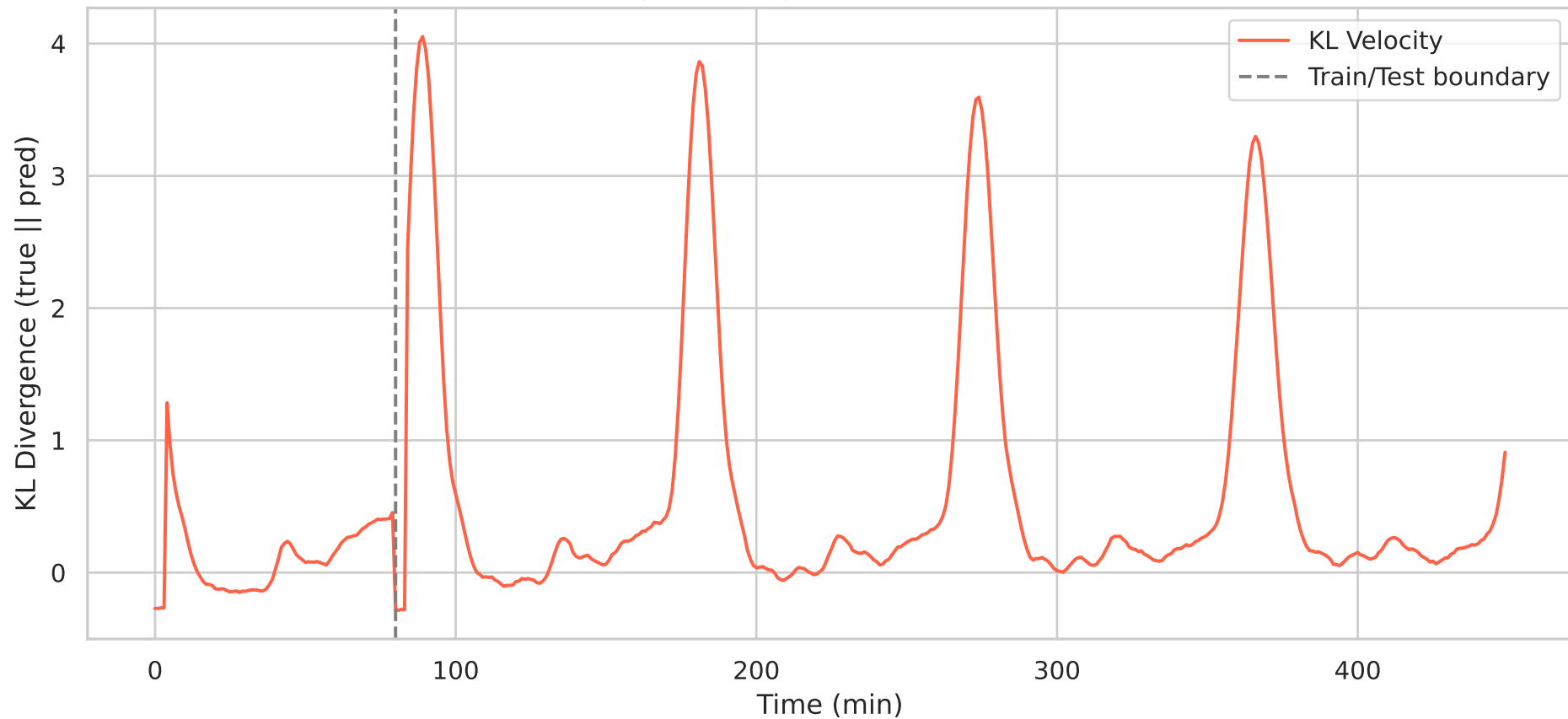
Final Velocity KL Divergence: lstm — Vel KL=0.9100
