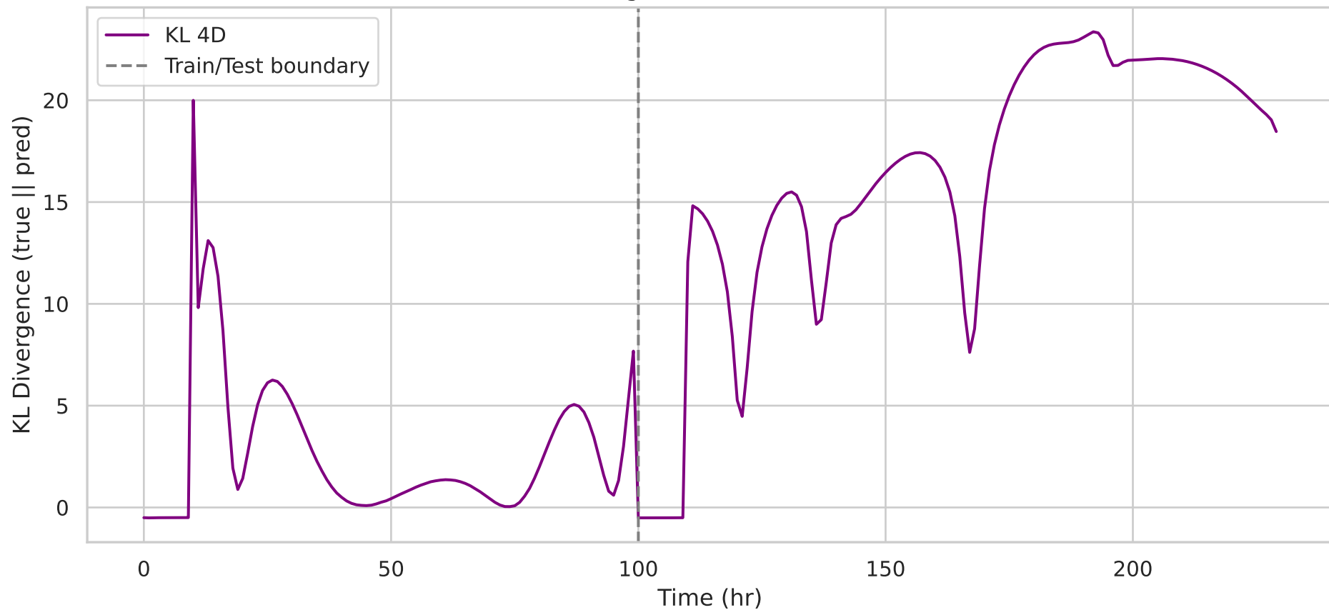
Full 4D KL Divergence: mamba — KL=18.4637
