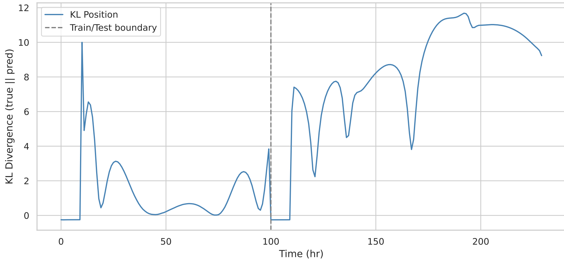
Final Position KL Divergence: mamba — Pos KL=9.2319
