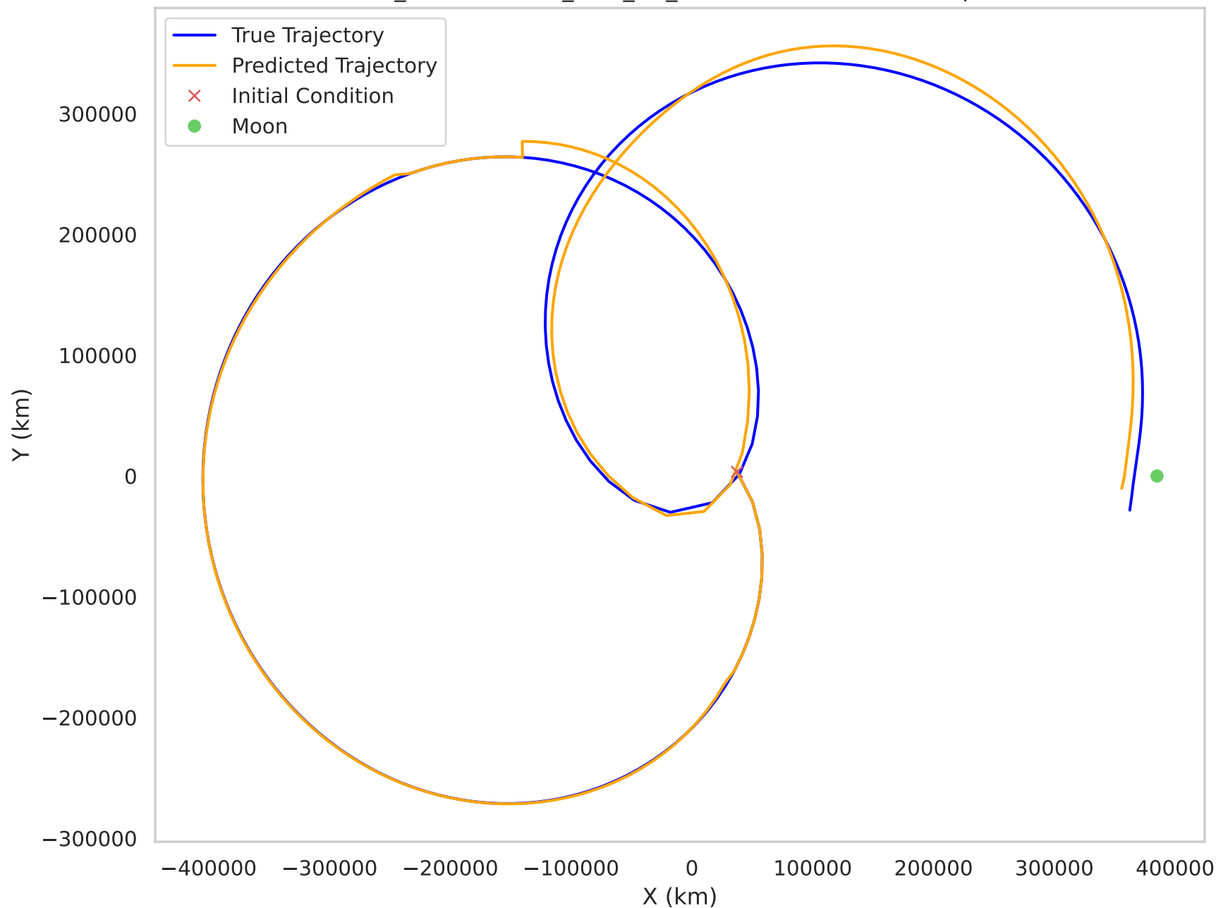
MAMBA Prediction for Trajectory 124 Orbit: 2.1_RETROGRADE_GEO_TO_MOON, Train Ratio: 0.1, Epochs: 10
