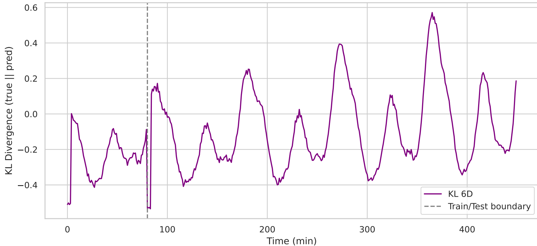
Full 6D KL Divergence: mamba — KL=0.1863
