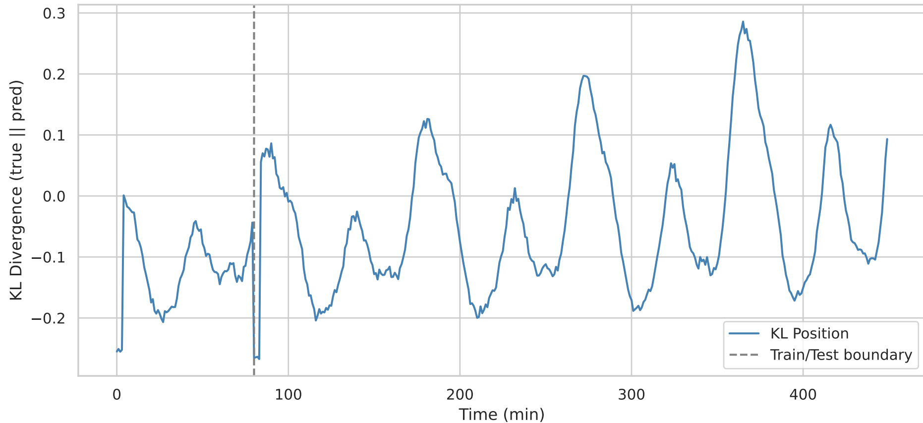
Final Position KL Divergence: mamba — Pos KL=0.0933
