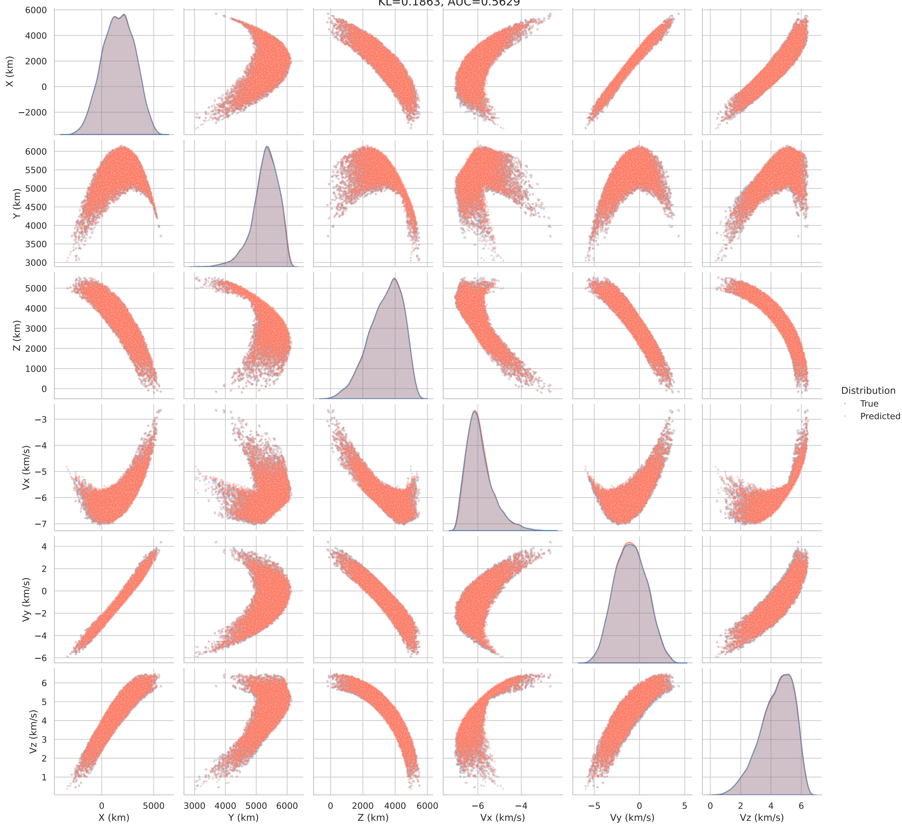
mamba Final State Pairplot — True vs Predicted KL=0.1863, AUC=0.5629
