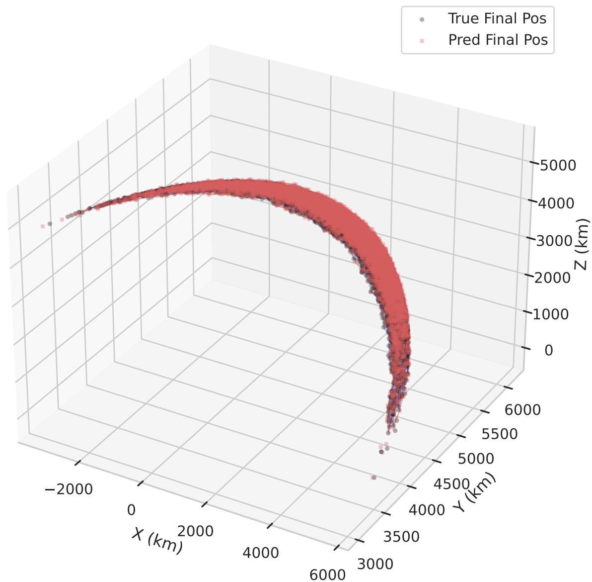
mamba Final State Positions Alpha Shape Vol Ratio (Pred/True): 1.8976
